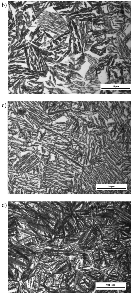
Fig. 1. Microstructure of ductile iron samples; a) DI, b) ADI 400_180, c) ADI 370_180, d) ADI 320_180
