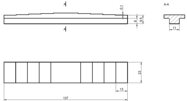
Fig. 2. Pictorial drawing of the sample
