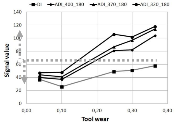
Fig. 4. Signal of cutting force -F_z in the 2 nd second of cutting for different DI samples
