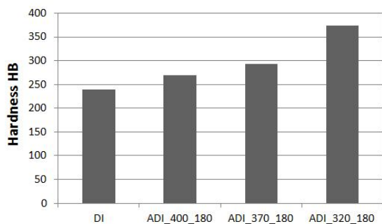
Fig. 9. Hardness of the tested DI and ADI samples
