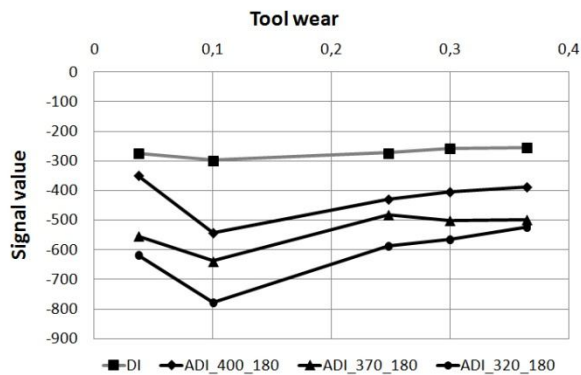
Fig. 5. Signal of acoustic emission –Ae min. for different DI samples
