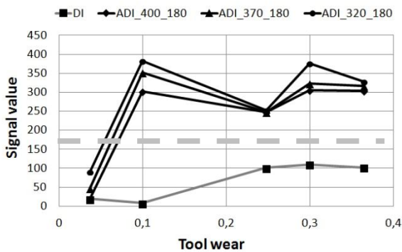
Fig. 6. Signal of acoustic emission –Ae mod. in the 2 nd second of cutting for different DI samples
