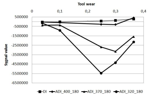
Fig. 8. Signal of vibration –Vz mom3 for different DI samples
