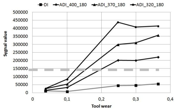
Fig. 7. Signal of vibration –Vz mom2 for different DI samples
