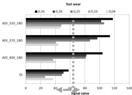
Fig. 3. Signal of cutting force -F_z in the 2 nd second of cutting for different DI samples
