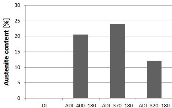
Fig. 10. Austenite content in samples of the tested DI and ADI
