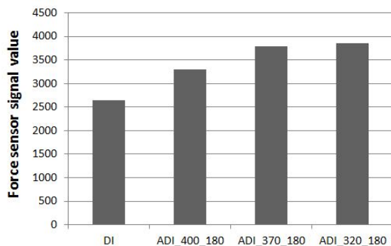
Fig. 11. Changes in values of the signal of the cutting force F_{z_{max}} recorded for the maximum tool edge wear of 0,36
