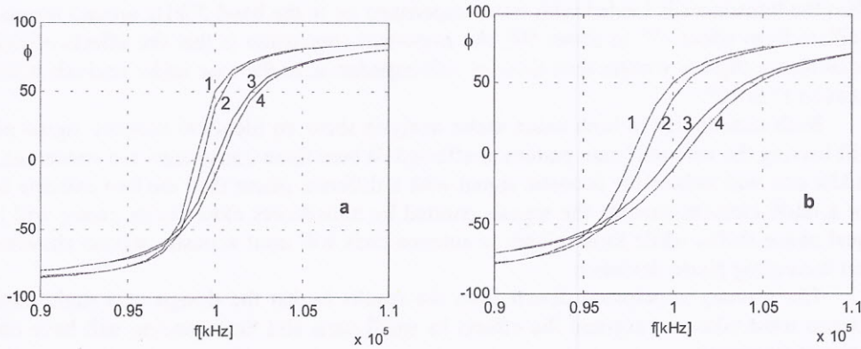
Fig.4 The effects of self and mutual impedance on phase shift of the acoustic signal a) one-sided load of the transducer, b) two-sided load of the transducer, line: 1 - for self impedance load excluding mutual radiation, 2 - for loads that are the result of self and mutual impedance, 3 - for acoustic impedance loads (plane wave), 4 - for acoustic impedance load (plane wave including mutual impedance).
