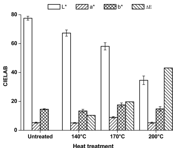
Fig. 2. L*a*b* values of untreated and thermally treated samples with the standard deviations of measurements
