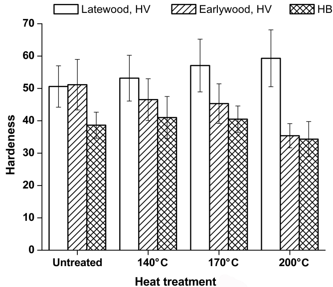
Fig. 8. Histogram of Vickers and Brinell hardness tests of untreated and thermally treated samples
