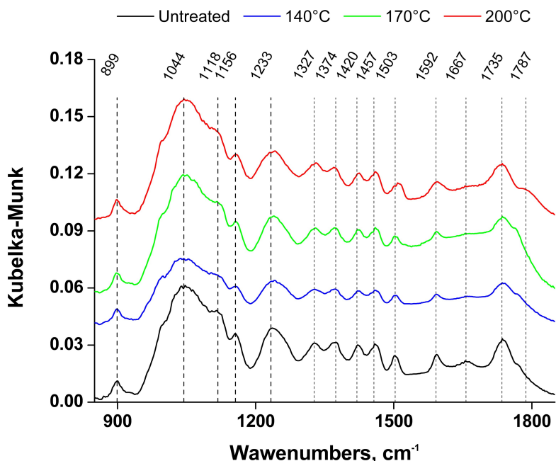
Fig. 9. FT-IR spectra of untreated and thermally treated wood samples. Focus on the 850-1850 \text{cm}^{-1} region
