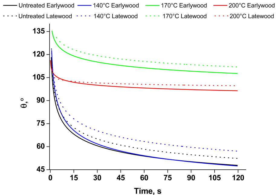
Fig. 6. Trends of the contact angles as function of time after water drop application
