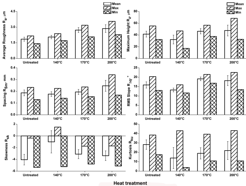
Fig. 4. L Roughness parameters obtained for measurements perpendicular to wood grain at the different heat treatments
