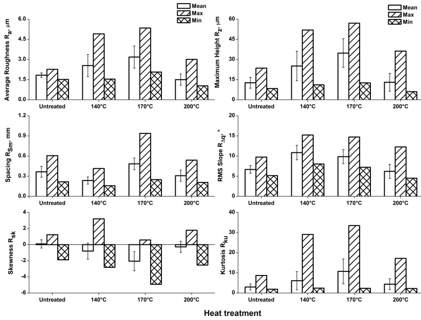
Fig. 3. Roughness parameters obtained for measurements parallel to wood grain at the different heat treatments
