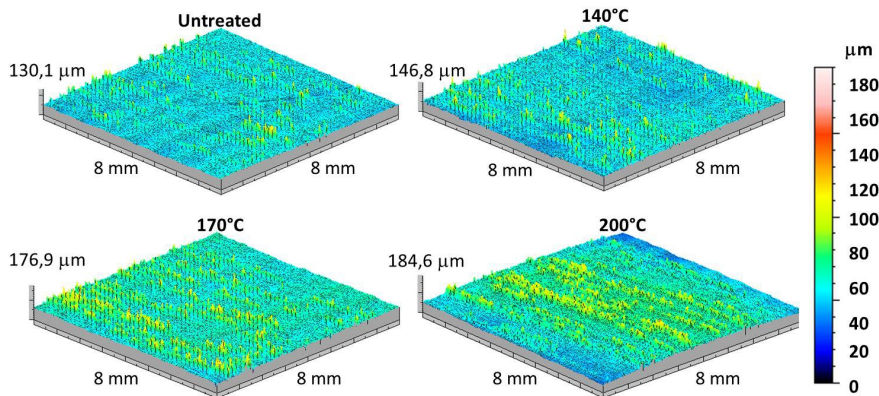
Fig. 5. 3D roughness maps of untreated and thermally treated sample surfaces, obtained for 8x8 mm areas
