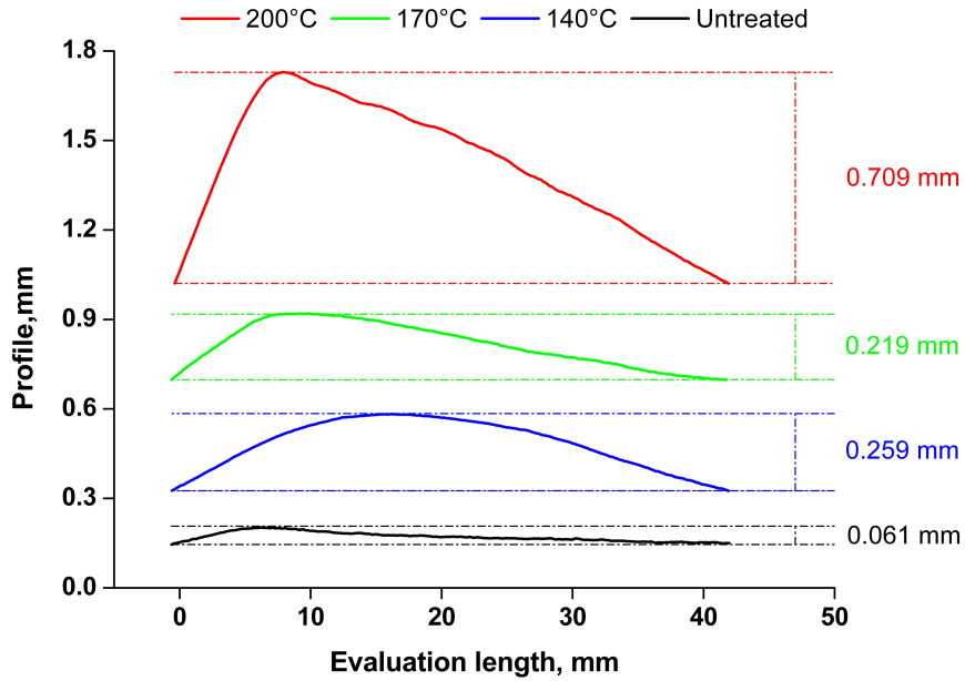
Fig. 7. Surface curvature profiles of untreated and thermally treated samples
