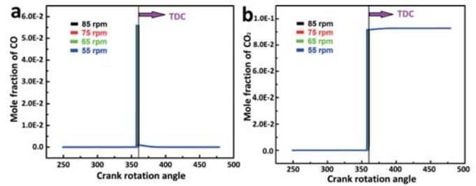
Fig. 9. (a) Effect of decreasing engine speed on \text{CO} emissions. (b) Effect of decreasing engine speed on \text{CO}_2 emissions.
