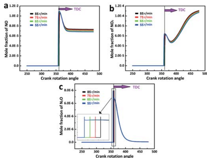
Fig. 4. (a) Effect of decreasing engine speed on NO emissions (b) Effect of decreasing engine speed on NO 2 emissions (c) Effect of decreasing engine speed on N 2 O emissions
