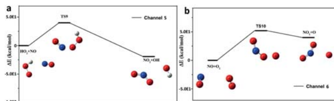
Fig. 7. (a) The optimized energy and geometries of reactant, transition state, and products for reaction P3 (b) The optimized energy and geometries of reactant, transition state, and products for reaction P4
