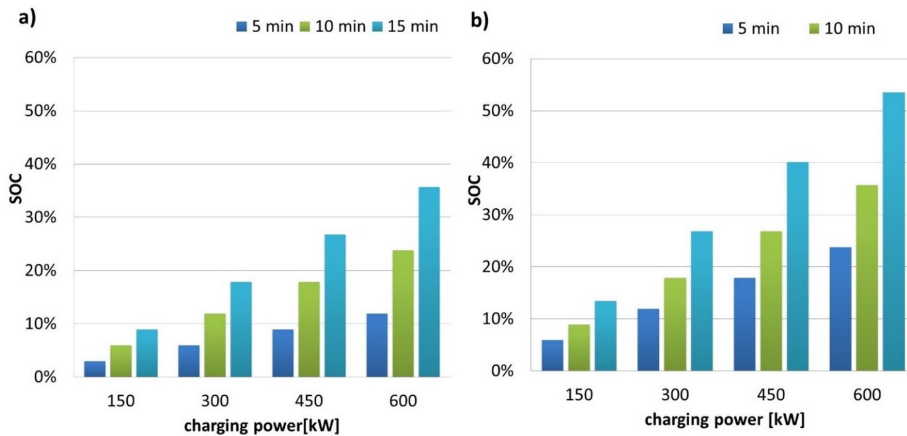
Fig. 6. Percentage of energy stored in the battery during charging of the battery with an energy capacity of a) 300 kWh, b) 200 kWh
