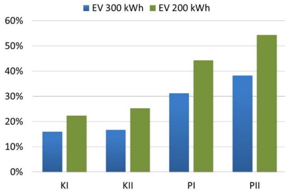
Fig. 5. Percentage share of energy taken from the battery
