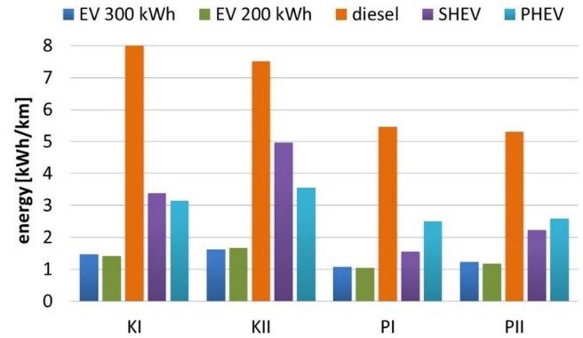
Fig. 3. Energy consumption
