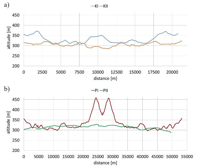
Fig.1. Vertical shape of terrain for a) urban and b) suburban routes
