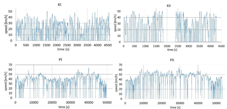
Fig. 2. Speed profiles of driving cycles
