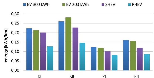
Fig. 4. Regenerated energy level
