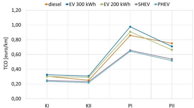
Fig. 7. Summary of Total Cost of Ownership (TCO) on selected bus routes
