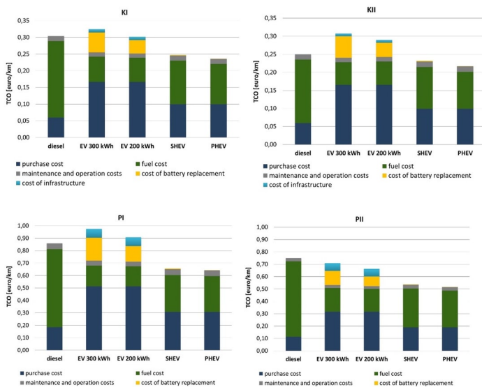
Fig. 8. TCO structure for the analyzed bus routes
