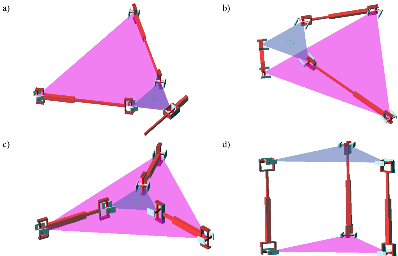
Fig.4. Examples of singular configurations of MT-3-UPU mechanism for direct and inverse kinematics problems: a) for q_1=0 , b) for \beta_1 = \pi/2 , c) for \alpha_i=0 ( i=1, 2, 3 ), d) for \alpha_i, \beta_i = 0 ( i=1, 2, 3 ).
