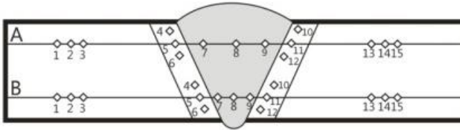
Fig. 3. Scheme of hardness measurements
