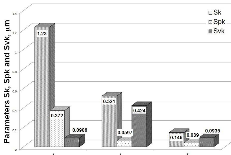
Fig. 7. Distribution of Sk, Spk and Svk parameters for hard turned, burnished and superfinished surfaces. 1-HT; 2-HT+B; 3-HT+SF
