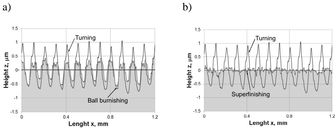
Fig. 4. Examples of surface profiles produced in sequential machining operations: a) HT+BB, b) HT+SF
