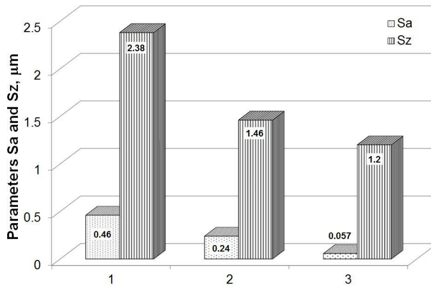
Fig. 3. Comparison of Sa and Sz roughness parameters for HT (1) HT+B (2) and HT+SF (3) sequences
