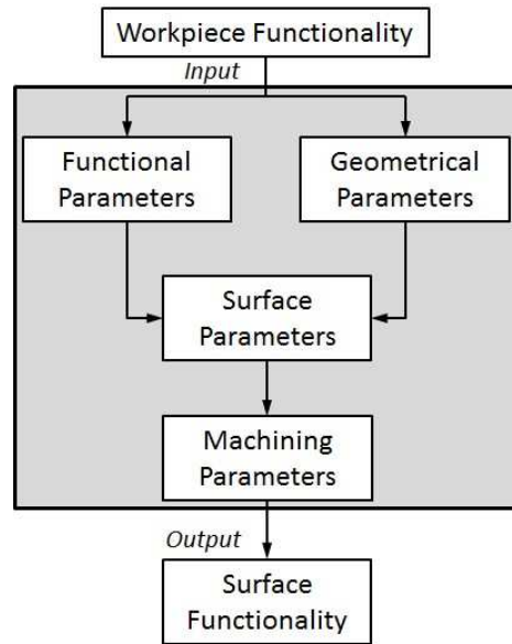
Fig. 1. Relationship between surface functionality and process parameters [2]
