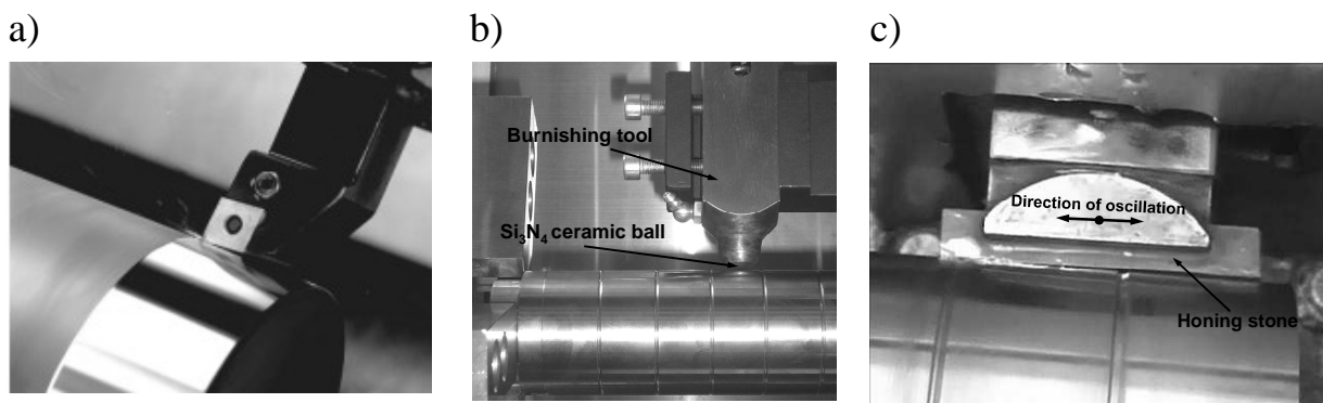
Fig. 2. Three machining operations used in the technological sequences tested in this study: a) hard turning, b) ball burnishing, c) superfinishing
