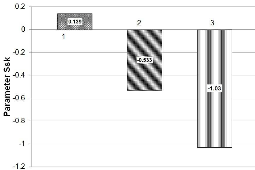
Fig. 8. Values of skewness Ssk for hard turning and burnishing operations. 1-HT; 2-HT+B; 3-HT+SF
