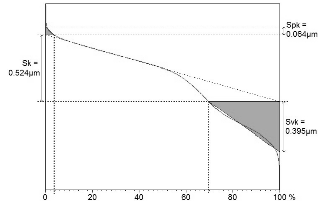
b) HT+B (Sr1=3.43%, Sr2=69.7%)
