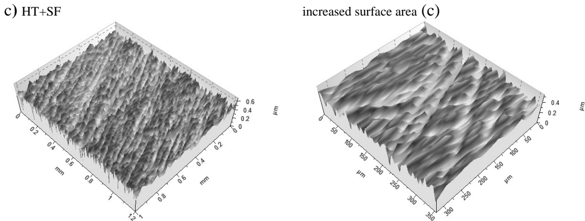
Fig. 5. Surface textures produced in dry hard turning (a), burnishing (b) and superfinishing (c) operations
