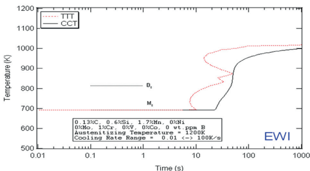
Fig. 1. Phase diagram for overlay welded metal with reference electrode type E300
