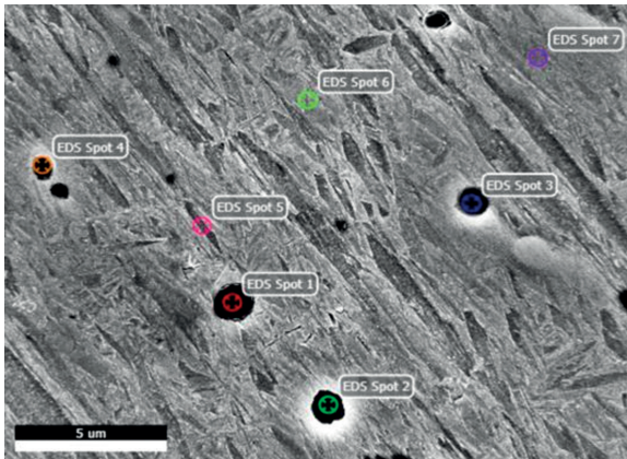
Fig. 7. SEM image of layer modified with TiN + Cr
