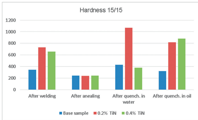
Fig. 10. Hardness after heat treatment
