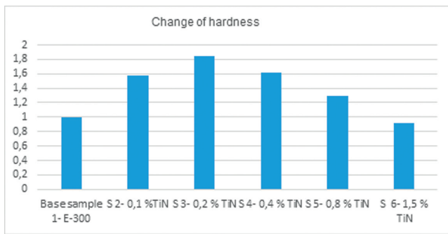
Fig. 9. The change of hardness dependence on the TiN content
