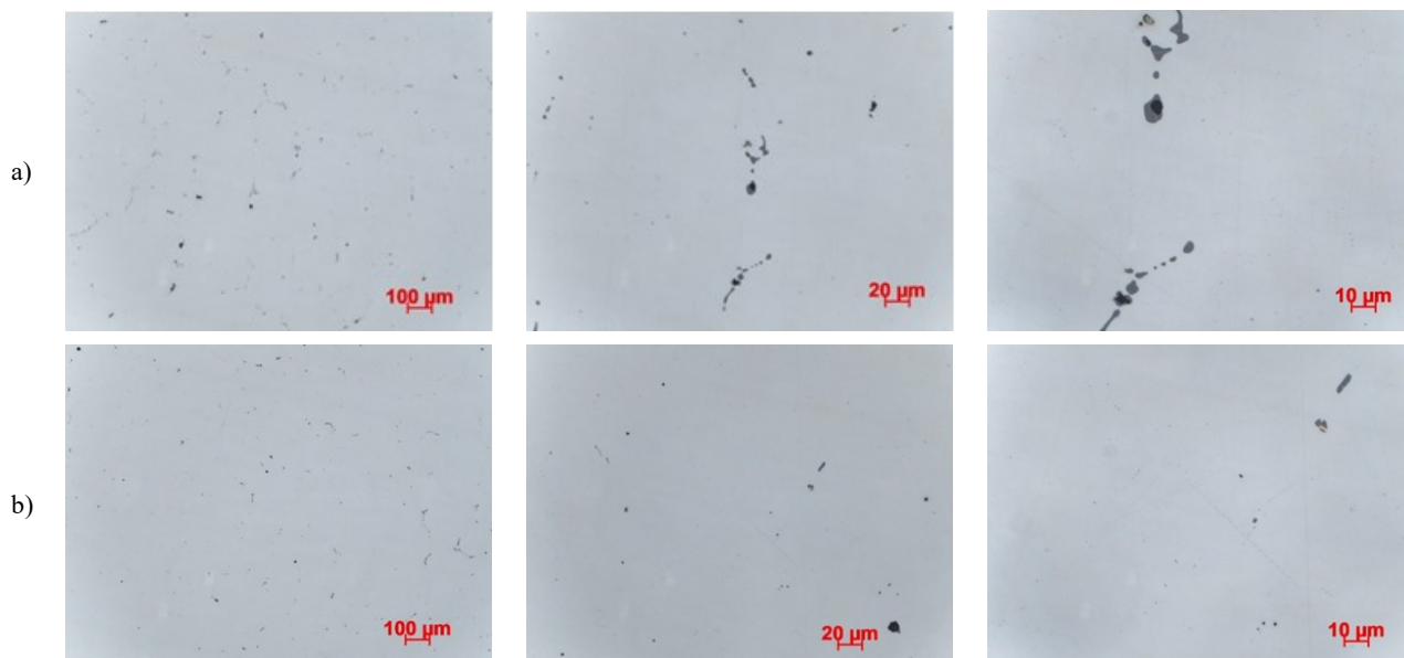
Fig. 1. Microstructure of LCC cast steel (unetched polished section): a) before filtration; b) after filtration
