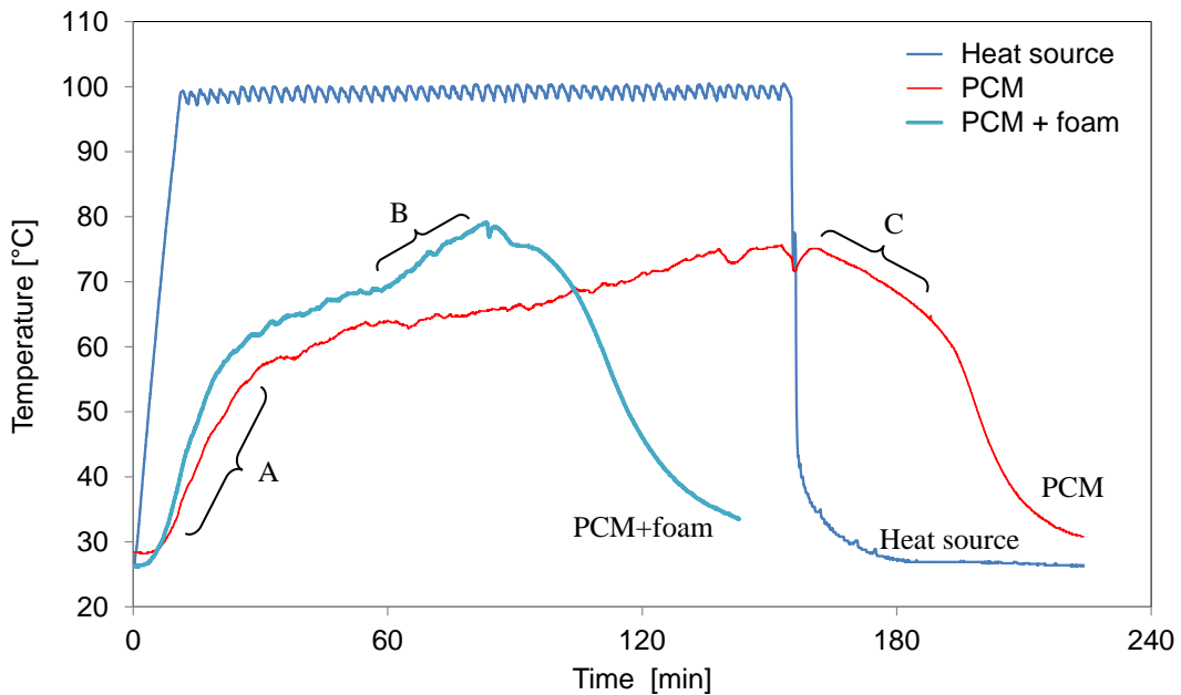
Fig.2. Temperature profiles for water heat source (Heat source) in the heat accumulator (distance of 20mm from the heat source) with only PCM paraffin (PCM) and with embedded in PCM metal cellular Zn-Al structure (PCM + foam). Distance A corresponds to preheating period of PCM (paraffin) to the melting point, B - to preheating of molten PCM, C – solidification of molten PCM.
