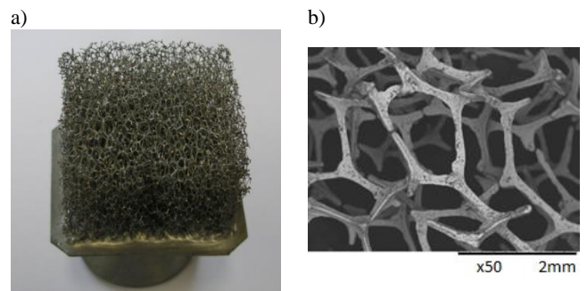
Fig. 1. View of cellular Zn-Al metal foam attached to the plate (a), open cell porous structure with some misruns (b)
