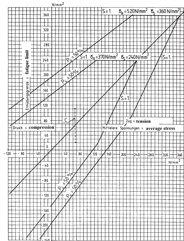
Fig. 4. A Goodman diagram illustrating the fatigue strength for non-welded elements made of S235JR and S355J2 steel [1]: P_u – survival probability, \sigma_R – tensile strength, \sigma_S – yield point
