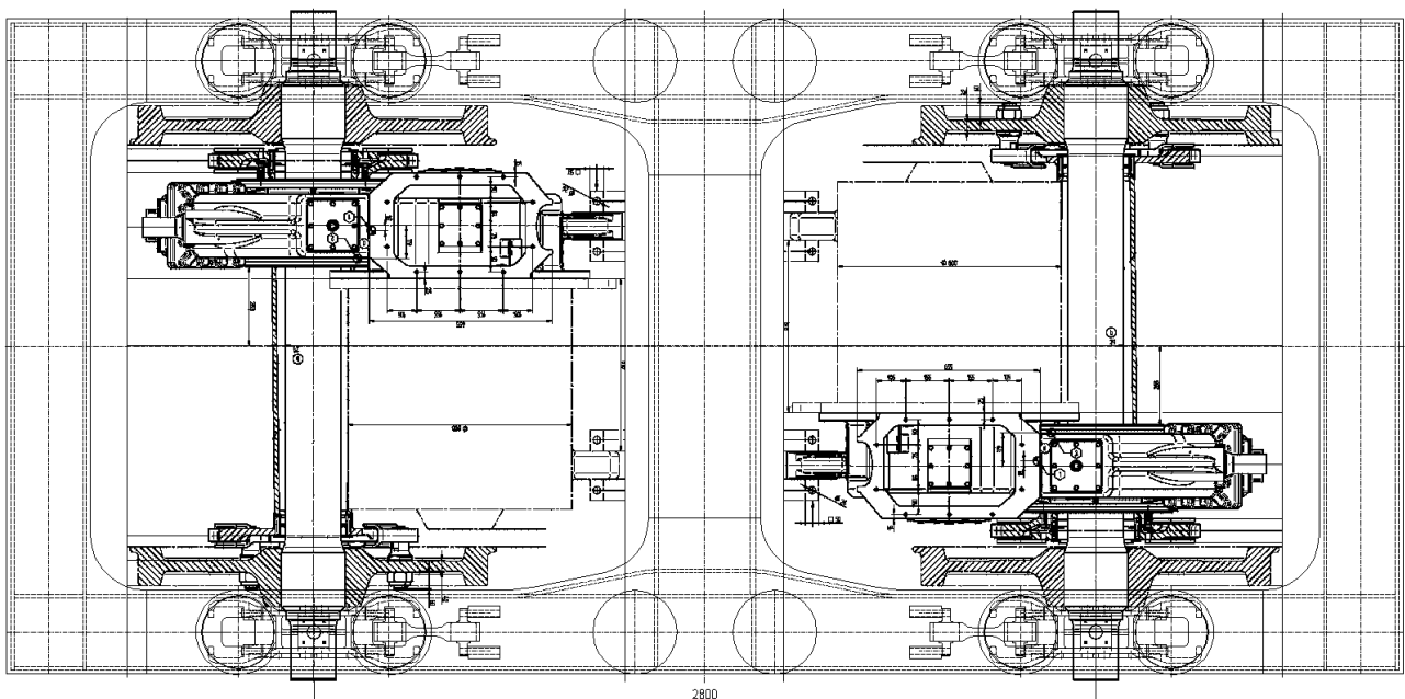
Fig. 3. An example of a review of the development of a drive system using 2D design software [authors' own work]
