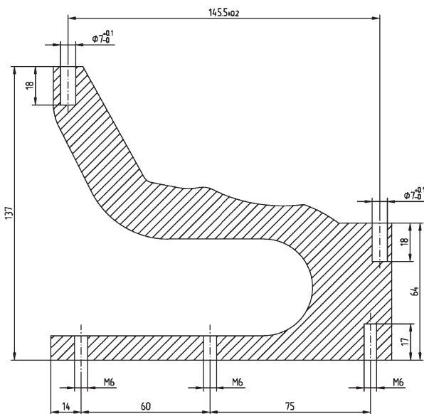
Fig. 8. A fine part designed in 2D software, acting as an “input” for a CNC machine tool [authors’ own work]
