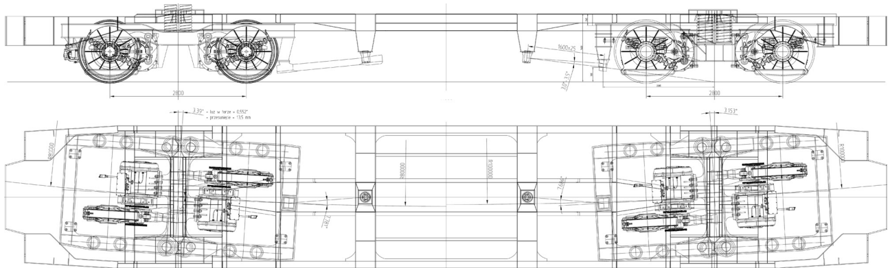
Fig. 2. An example of a 2D analysis performed using 2D design software [own elaboration]
