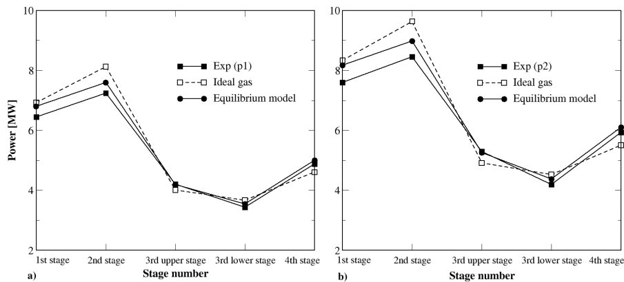
Figure 5. Low pressure part power output calculated conditions at: a) point 1, b) point 2.
