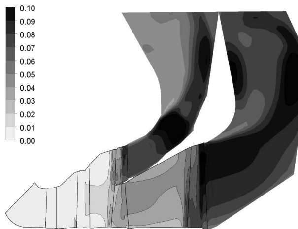
Figure 4. Wetness level (%) calculations for data point 1.
