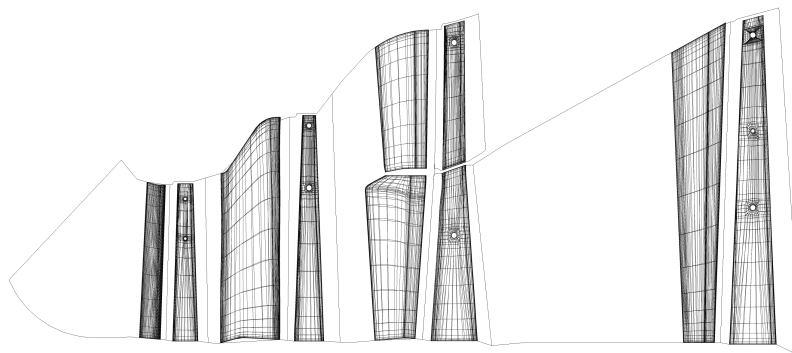
Figure 2. Numerical geometry of 13K215 LP part with Baumann stage.
