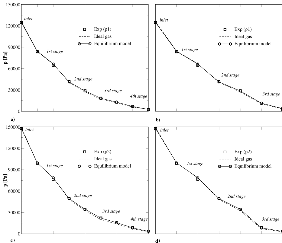
Figure 3. Pressure drop for data set point 1 throughout the: a) lower part, b) upper part, calculations for point 2, c) lower part, d) upper part.
