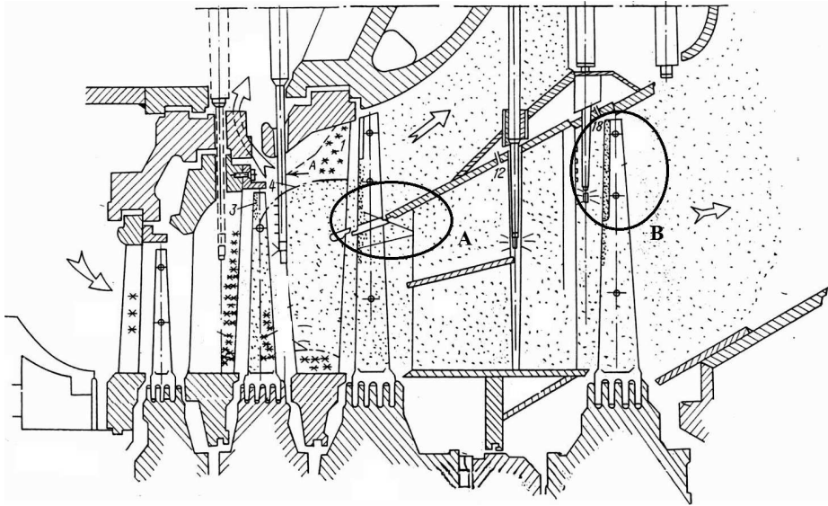
Figure 1. Low pressure part of 13K215 turbine, regions of increased corrosion: A – conical visor, B – last stage blades tips.
