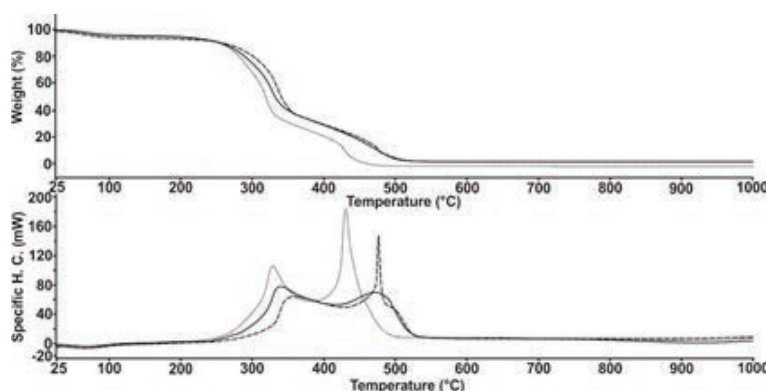
Fig. 1. Thermal analysis - TG/DSC (chipboard – solid line, plywood – dashed line, wood chips – dotted line, H.C. – heat capacity)
