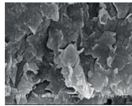
SEM diagram of clay at 17.1-17.3m depth
