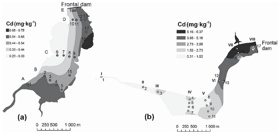
Fig. 5. Spatial distribution of Cd in bottom sediments of the reservoirs: Zalew Zemborzycki (a) and Brody Iłżeckie (b)
