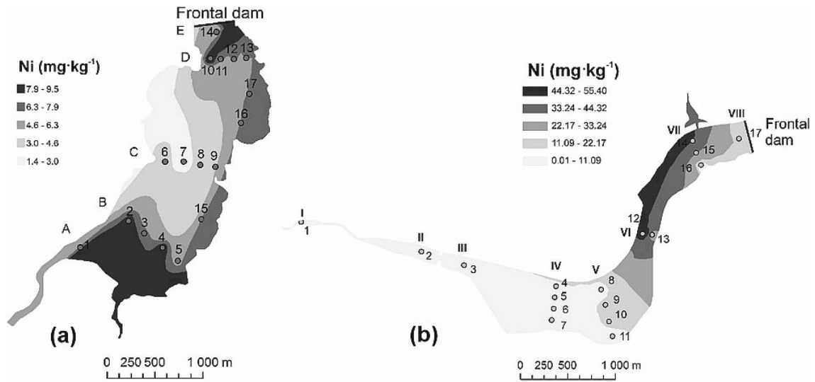
Fig. 8. Spatial distribution of Ni in bottom sediments of the reservoirs: Zalew Zemborzyccki (a) and Brody Iżeckie (b)
