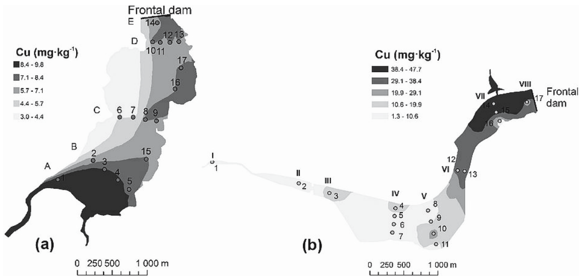
Fig. 6. Spatial distribution of Cu in bottom sediments of the reservoirs: Zalew Zemborzycki (a) and Brody Iłżeckie (b)
