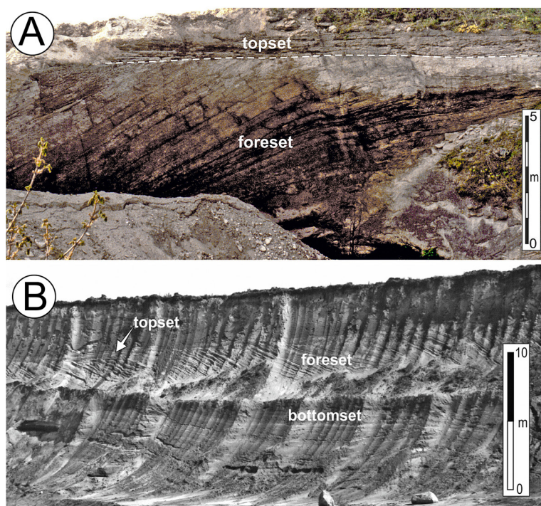
Fig. 1. Lithosomes with subfacies of Gilbert-type delta: A – Miocene marine calcarenites near Staszów (southern Poland); B – Pleistocene glaciolacustrine deposits in Bełchatów brown-coal mine (central Poland).
