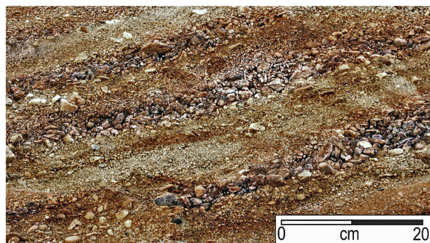
Fig. 4. Gravelly foresets deposited from coarse-grained subaqueous avalanches – the grain falls. Świdnica area, Sudetes Mts foreland, southern Poland.
