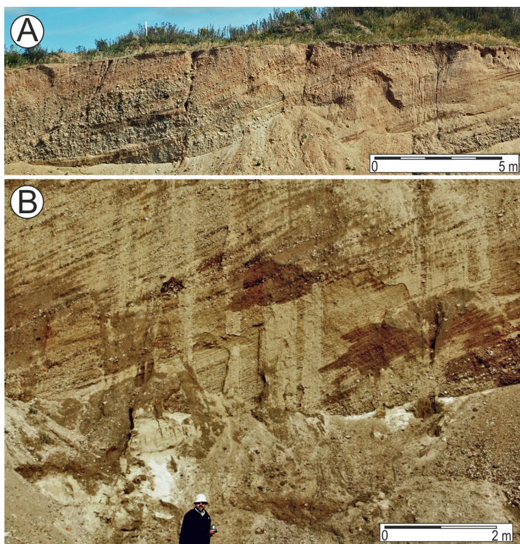
Fig. 3. Foresets of the Pleistocene glaciolacustrine Gilbert-type deltas. Both sites are located in the foreland of Sudetes Mts (southern Poland). Advancing ice sheet dammed deep lakes in foremountain valleys outflowing towards the glacier. A – Variable dip and grain-size of foresets prove that delta progradation took place in successive phases (photo P. Migoń).
