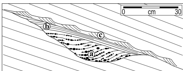
Fig. 6. The scour eroded by hydraulic jump on delta slope (based on Massari, 1996). a – Gravelly sand with backset cross-stratification (supercritical deposition), b – Horizontally stratified sand (upper plane bed), c – Horizon of ripples (lower flow regime).
