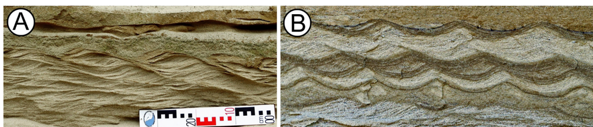
Fig. 7. Bottomset facies of distal prodelta (Bełchatów, central Poland). Fine-grained sands derived from climbing ripples. A-type climbing cross-lamination (A) was formed from some faster current than B-type lamination (B). A-type structure records the predomination of traction over suspension transport, and B-type structure proves deposition purely from suspension. On both photos the rippled bed is overlain by silty layer.
