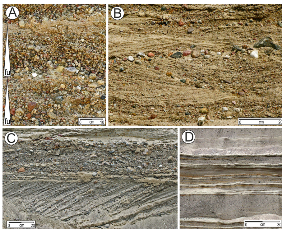
Fig. 2. Typical topset lithofacies (Pleistocene, Bełchatów, central Poland): A – Massive gravels of sheetflow origin, fining-up tendency (fu) is marked; B – Gravelly sand with trough cross-stratification derived from three-dimensional dunes; C – Gravelly sand with tabular cross-stratification derived from transverse bar, massive sandy gravel of diffuse gravel sheet above; D – Two thick beds of massive and poorly stratified gravelly sands derived from longitudinal bars.
