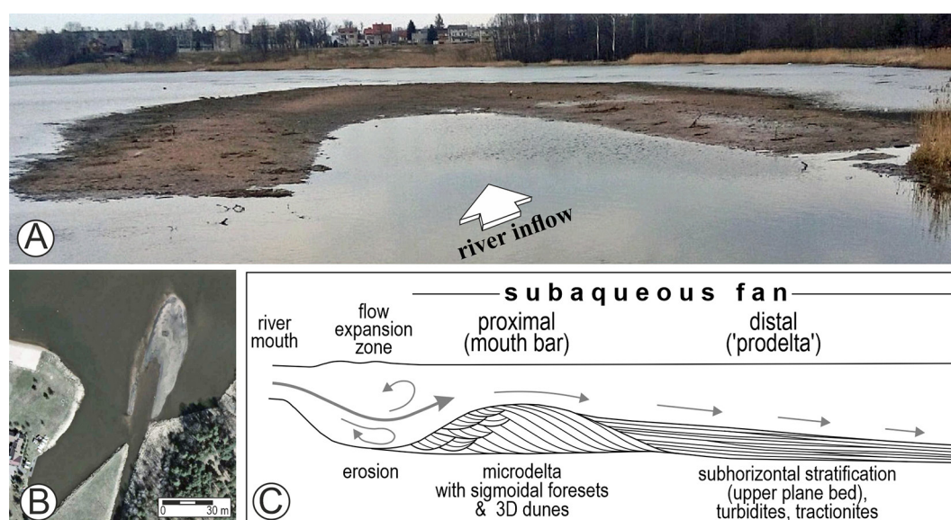
Fig. 10. Subaqueous fans: A, B – real photos; C – theoretical model. Both photos by Przepióra et al. (2019). Model draft partly based on Lang et al. (2017).
