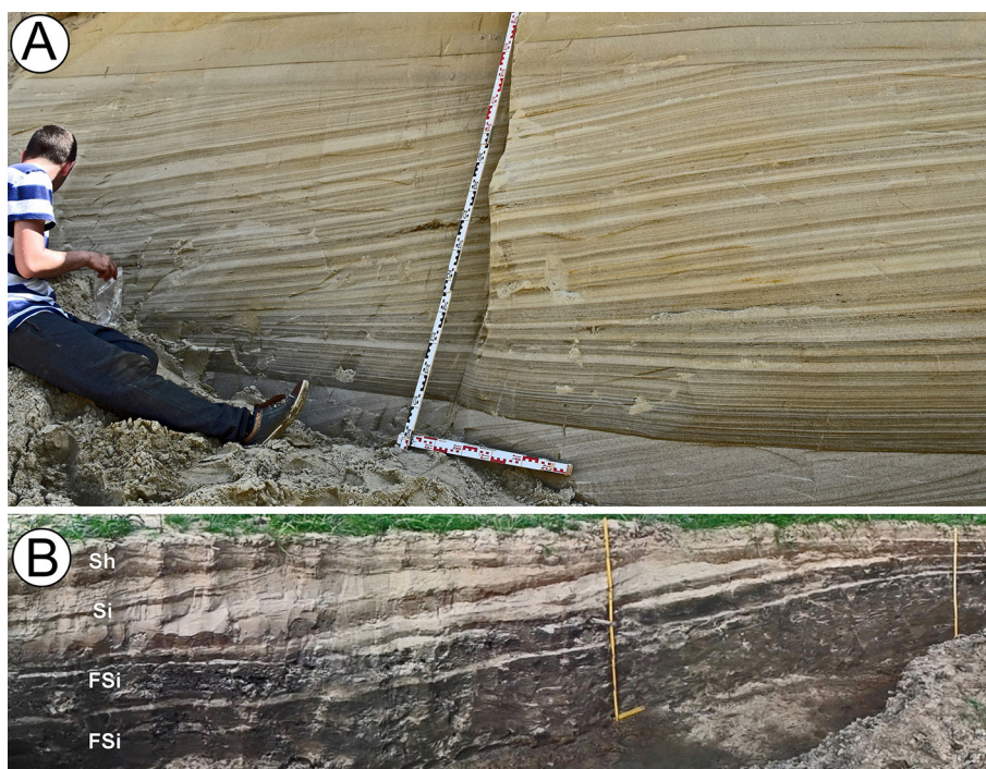
Fig. 8. Deposits of subaqueous fans. Low-angle stratification proves the gentle slope of fan. A – Light laminae are sandy and darker ones are sandy-silty (Ujście site in northern Poland, photo by M. Mleczak); B – Sands form light layers, and organic sandy silts form dark ones; scale bars are 1.5 m long (Suchedniów site in central Poland, photo from Przepióra et al., 2019).
