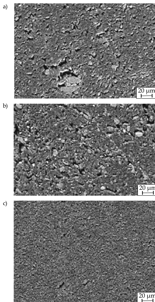
Fig. 1. SEM micrographs of brittle fracture surfaces of composites: a) K1, b) K2, c) K3
