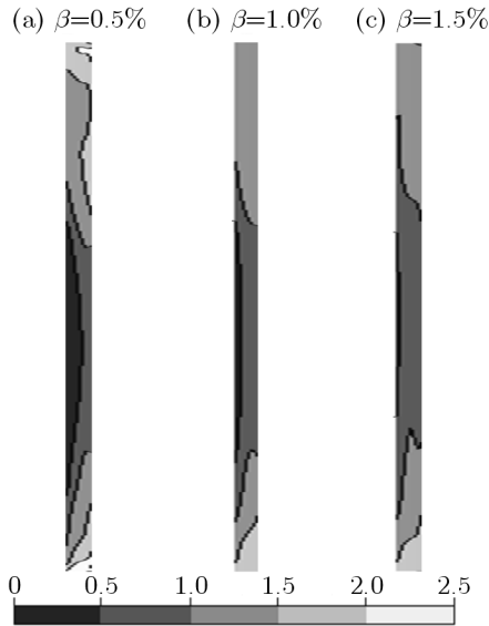
Fig. 11. Distribution of the mass flow on the inlet of SS4 slot
