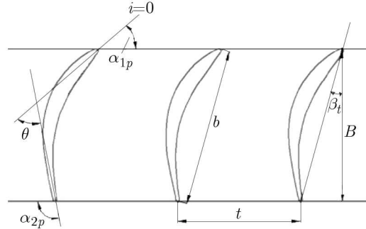
Fig. 1. The cascade and a selected blade profile
