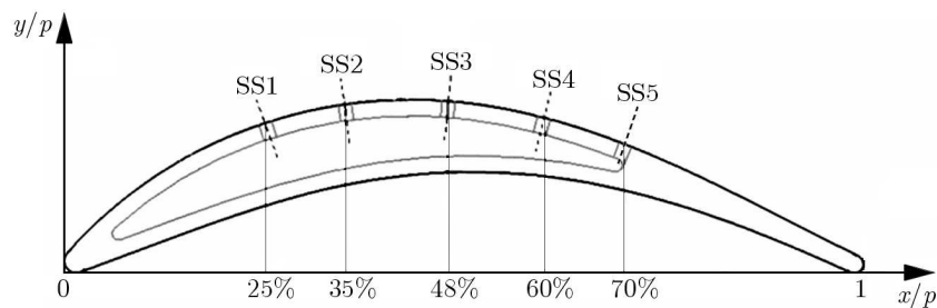
Fig. 3. Location of suction slots in calculation schemes
