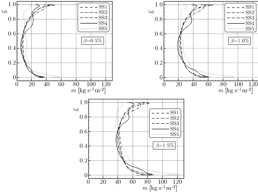
Fig. 10. Spanwise distribution of the suction flow rate at the suction slot inlet
