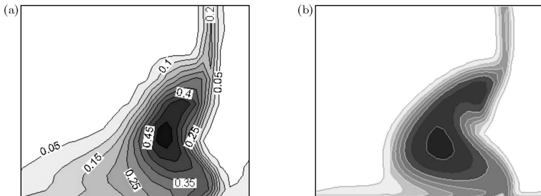
Fig. 5. Outlet total pressure loss; (a) experimental result, (b) calculation result
