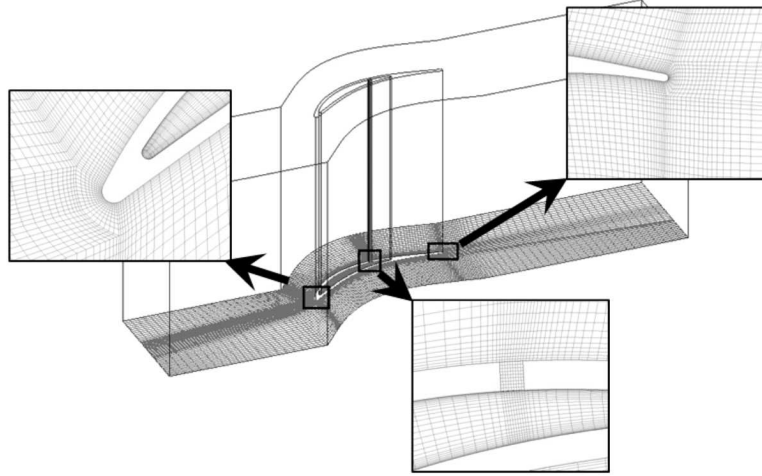
Fig. 2. Mesh for SS4 scheme computation
