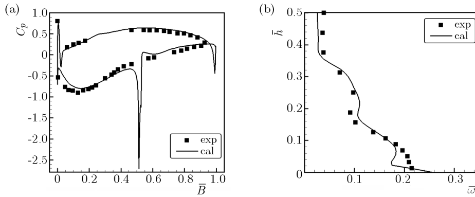
Fig. 4. (a) Static pressure coefficient; (b) total pressure loss
