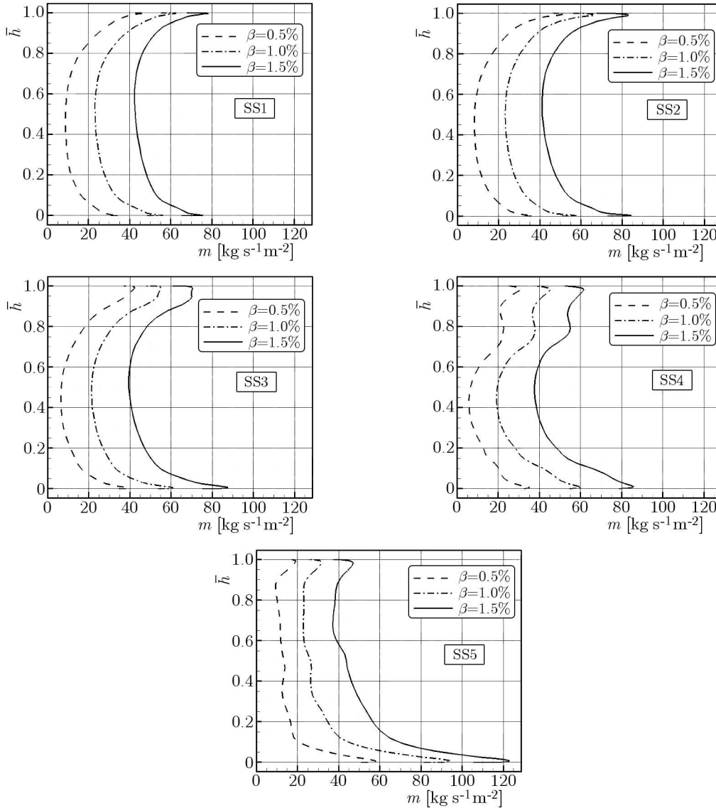
Fig. 9. Spanwise distribution of the suction flow rate under different configurations
