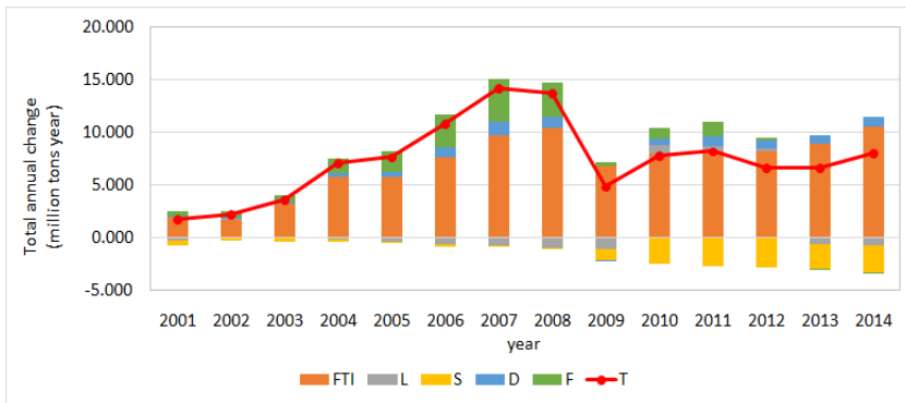
Fig. 4. SDA results - Net difference in total annual tonnage changes referred to 2000 and contribution of decomposition factors (millions of tons per year)
