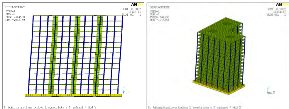
Fig. 4. First mode of the building with three cores - model VSB3
