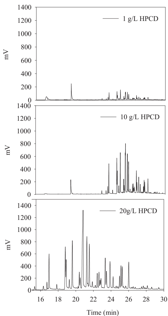
Fig. 3. Gas chromatogram at different HP- \beta -CD concentrations
