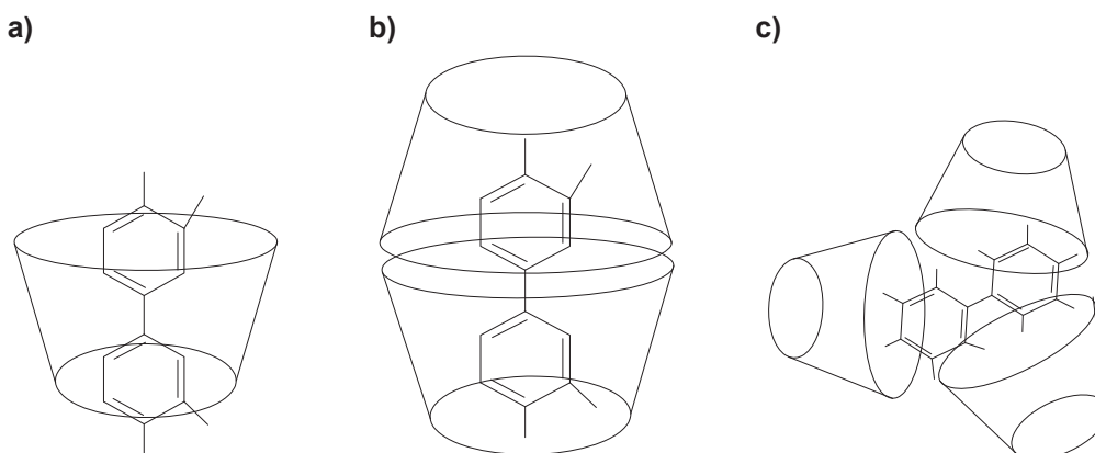
Fig. 4. Proposed inclusion forms of HP- \beta -CD – PCBs: a) cage model of single CD – PCBs; b) pipe model of two CD moleculars – PCBs; c) self aggregated CD moleculars – PCBs inclusions
