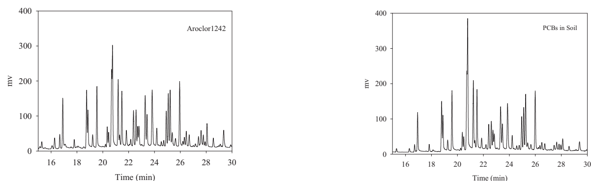
Fig. 1. Gas chromatogram of PCBs from standard and contaminated soil
