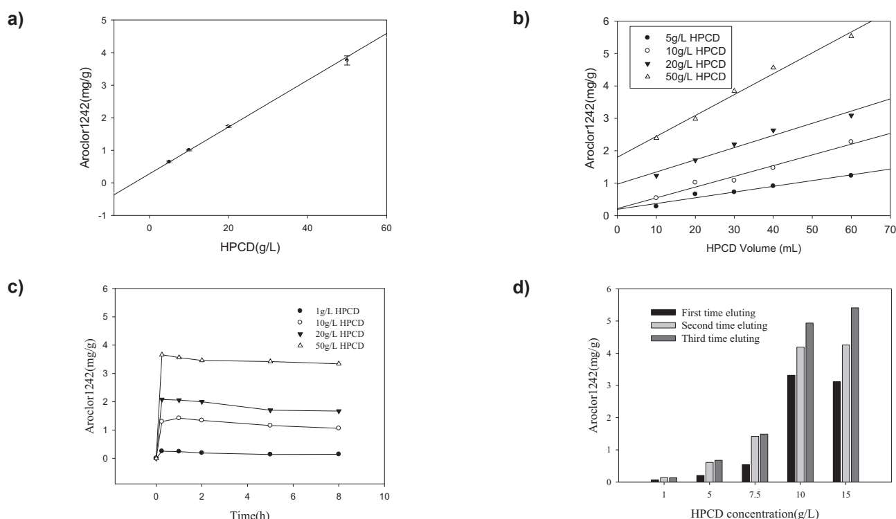
Fig. 2. a) Eluting of PCBs at different HP- \beta -CD concentrations; b) Eluting of PCBs at different HP- \beta -CD volumes; c) Effect of contact time on PCBs eluting; d) Effect of eluting cycles at different HP- \beta -CD concentrations
