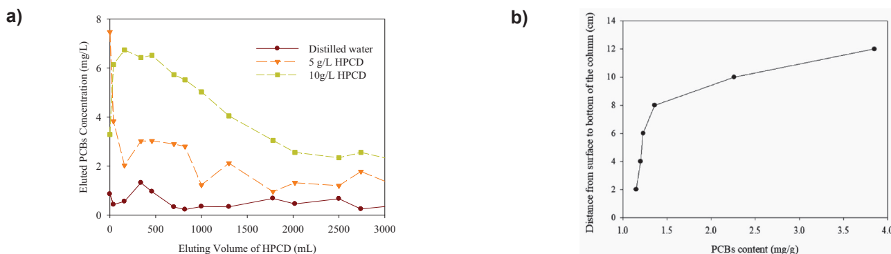
Fig. 6. a) Column eluting curve of PCBs from soil by HPCD; b) Mass distribution profiles of PCBs along the soil column depth
