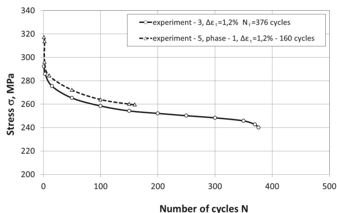
Fig. 3. Diagrams of cyclic deformation of the P92 steel in conditions of research experiments no. 3 and 5
