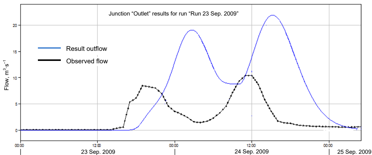
Fig. 4. Observed and simulated stream flow hydrographs for the calibration (23–25 September 2009) period; source: own study
