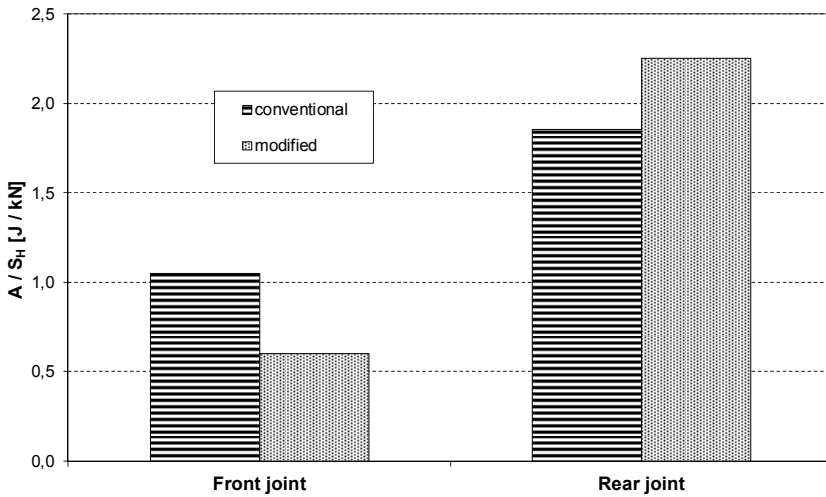
Fig. 10. Total relative friction work in the joints of chain links for \Delta p/p = 2.0\% , \mu^p = 0.2 , \mu^g = 0.15
