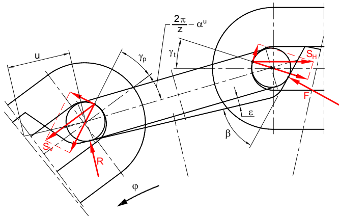
Fig. 2. Load on the horizontal link contacting the front torus with the seat bottom and rear torus with the side surface of tooth
