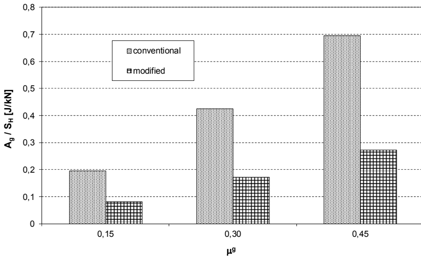
Fig. 7. Total relative friction work on the bottom of a modified drum and conventional drum for \Delta p/p = 0.5\% , ( \mu^p = 0.1 )
