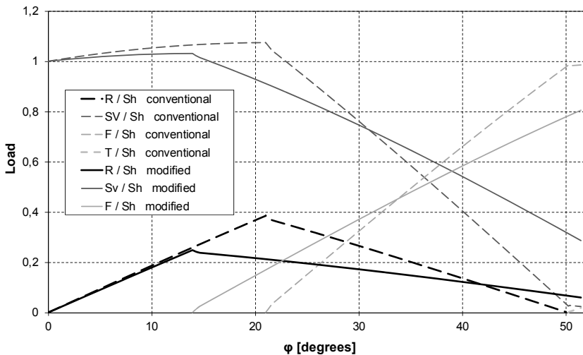
Fig. 4. Load curve of modified drum and conventional drum for \Delta p/p = 0.5\% , \mu^p = 0.1 , \mu^g = 0
