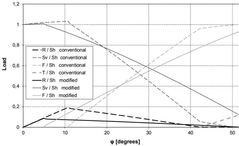
Fig. 6. Load curve of modified drum and conventional drum for \Delta p/p = 3.0\% , ( \mu^p = 0.1 ; \mu^s = 0 )
