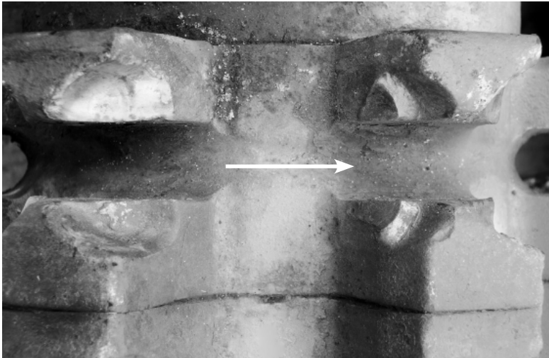
Fig. 1. Sprocket drum tooth with high degree of wear
