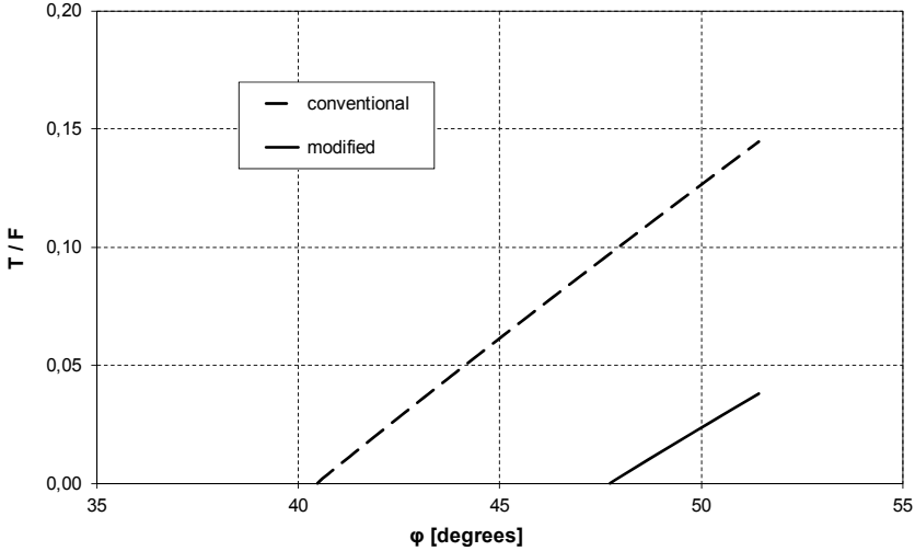
Fig. 9. Curve of the ratio of the forces T/F in conventional drums and modified drums for \Delta p/p = 3.0\% , \mu^p = 0.2 , \mu^g = 0.15
