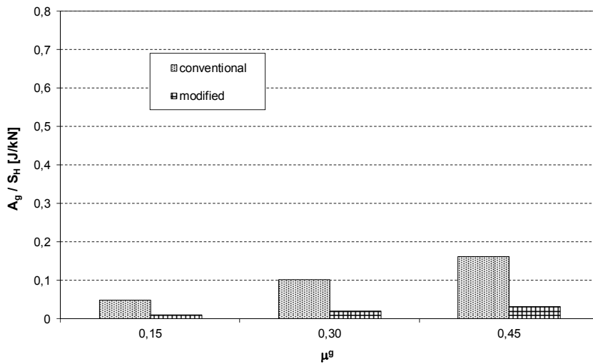
Fig. 8. Total relative friction work on the bottom of a modified drum and conventional drum for \Delta p/p = 3.0\% , ( \mu^p = 0.1 )
