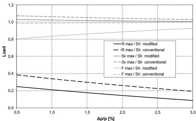
Fig. 5. Influence of elongation of links' pitches on the maximum values of the load ( \mu^p = 0.1 ; \mu^s = 0 )
