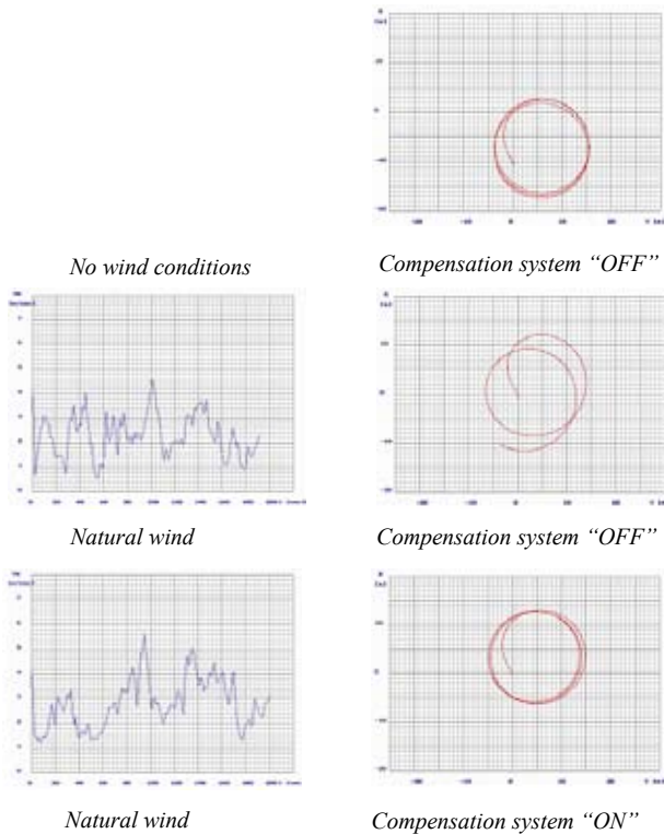
Fig. 4. Examples of the turning tests
