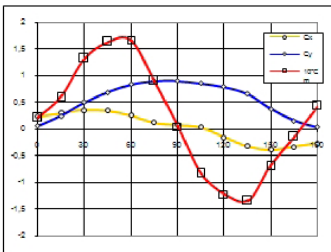
Fig. 2B Aerodynamic characteristics of ship model M467 with the wind simulation system [3]
