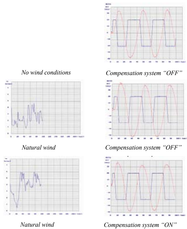
Fig. 5. Examples of the zigzag tests
