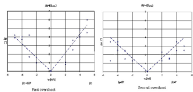
Fig. 7. Dependence of change of the first and second overshoot angles in zigzag tests on the wind angle and velocity
