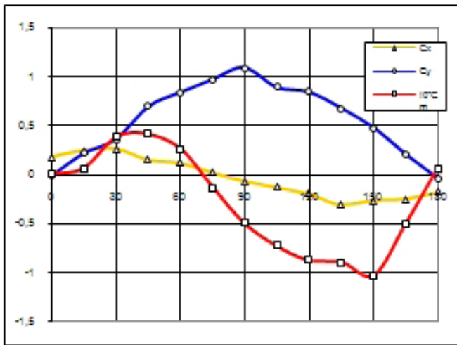
Fig. 2A Aerodynamic characteristics of ship model M509 [2]
