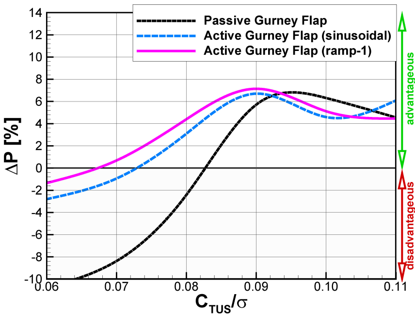
Fig. 23. Relative power reduction ( \Delta P ) vs. thrust coefficient ( C_{TUS}/\sigma ). Results obtained for the configurations: Passive Gurney Flap, Active Gurney Flap (sinusoidal) and Active Gurney Flap (ramp-1)
