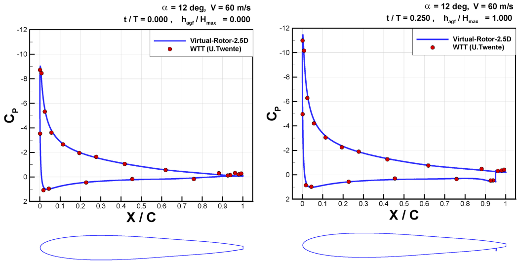
Fig. 12. Comparison of CFD and WTT results related to pressure-coefficient ( C_p ) distribution for AGF fully retracted (left) and fully deployed (right). \alpha=12 deg, V=60 m/s
