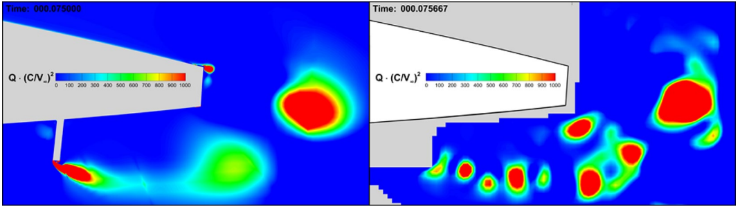
Fig. 8. Q-criterion contours at a moment of fully deployed AGF. Comparison of results of CFD (left picture) and WTT (right picture)
