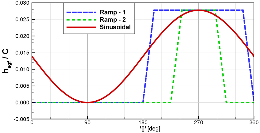
Fig. 17. Considered variants of AGF-motion schedules
