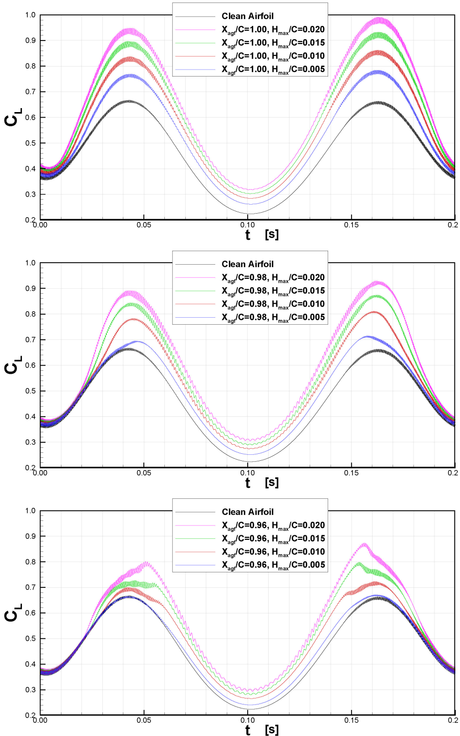
Fig. 14. Time-variable lift coefficient C_L captured during one period of oscillations, for the clean airfoil and for twelve configurations of airfoil equipped with oscillating AGF
