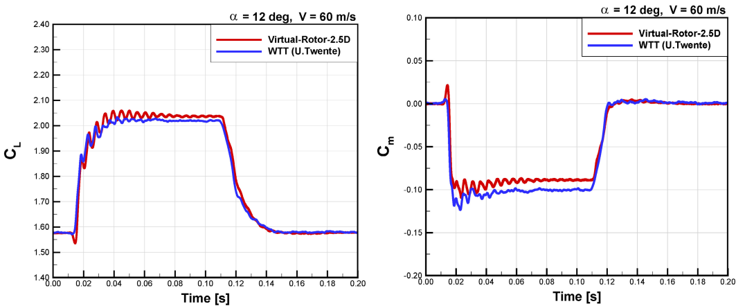
Fig. 10. Momentary lift coefficient ( C_L ) and pitching moment coefficient ( C_m ) vs. time (t). Comparison of CFD and WTT results. \alpha=12\text{deg} , V=60\text{m/s}
