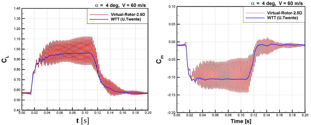
Fig. 6. Momentary lift coefficient ( C_L ) and pitching moment coefficient ( C_m ) vs. time (t). Comparison of CFD and WTT results. \alpha=4\text{deg} , V=60\text{m/s}
