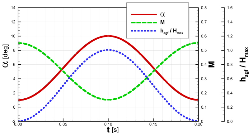
Fig. 13. Harmonic changes of angle of attack ( \alpha ), free stream Mach number ( M ) and deployment of AGF ( h_{agr} ) assumed in conducted 2D sensitivity analysis
