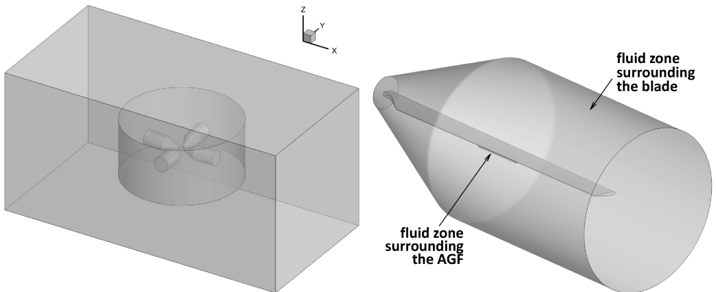
Fig. 3. Overall topology of computational mesh
