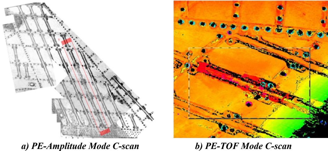
Fig. 6. Large delamination along the longeron of MiG-29's vertical fin
