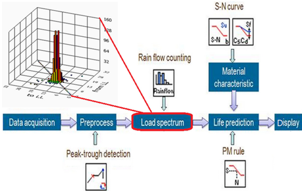
Fig. 21. A scheme for calculating fatigue life
