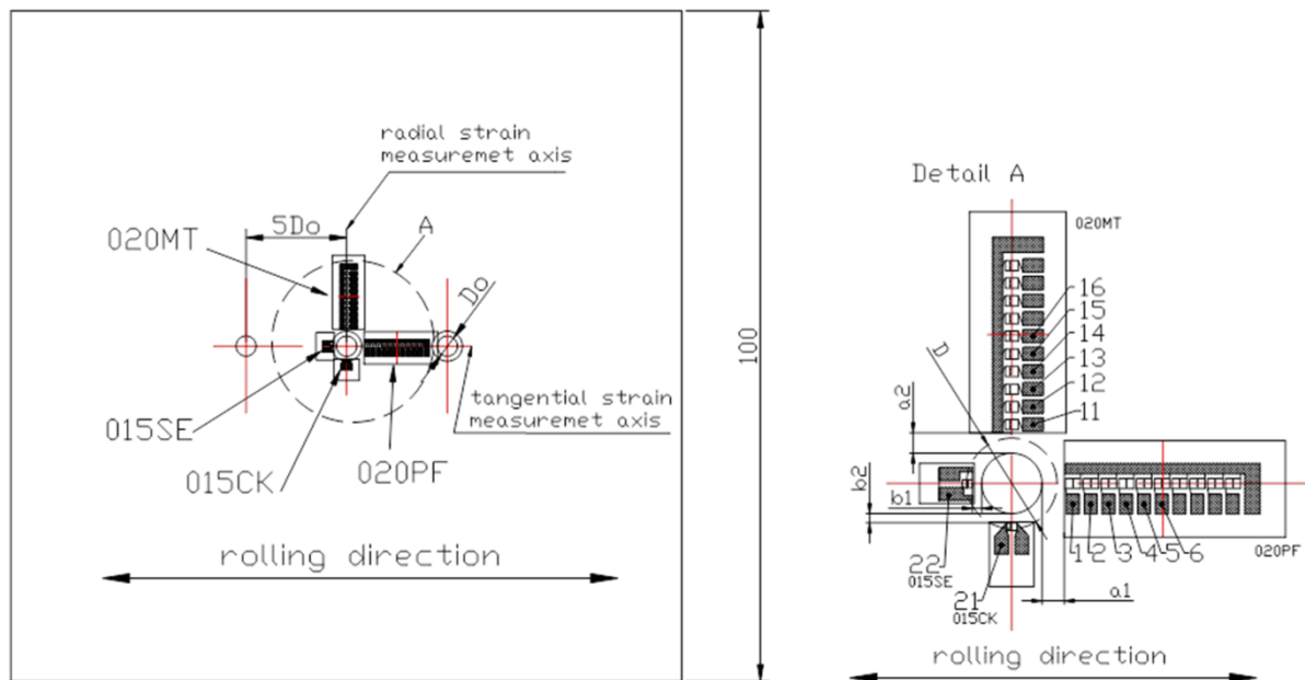
Fig. 13. Specimen geometry
