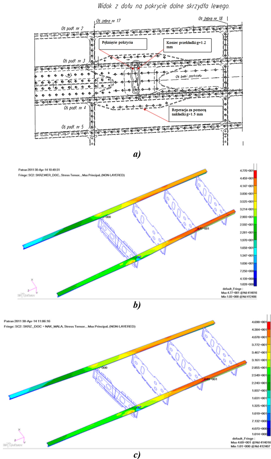
Fig. 12. The FEM analysis of a crack in the PZL M28 wing area of rib 17 during fatigue testing:
