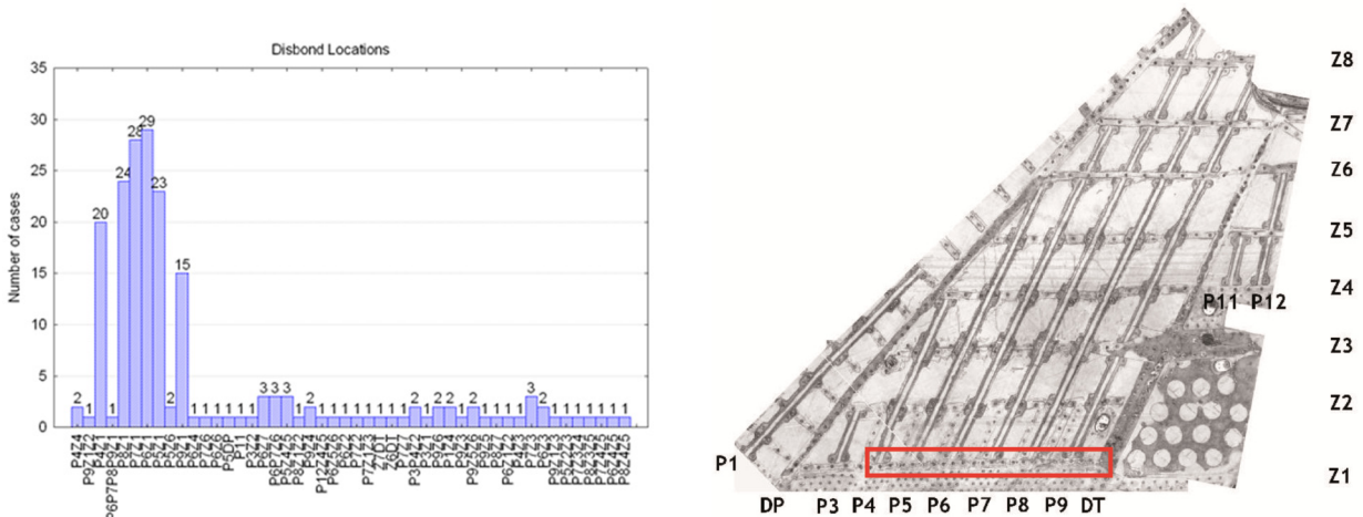
Fig. 9. Distribution of disbands in the MiG-29's vertical stabilizer
