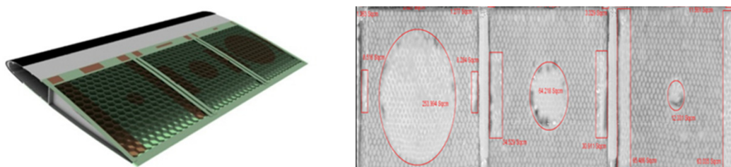
Fig. 2. Calibration specimen design (left) and MIA (right) inspection results of the disbonds
