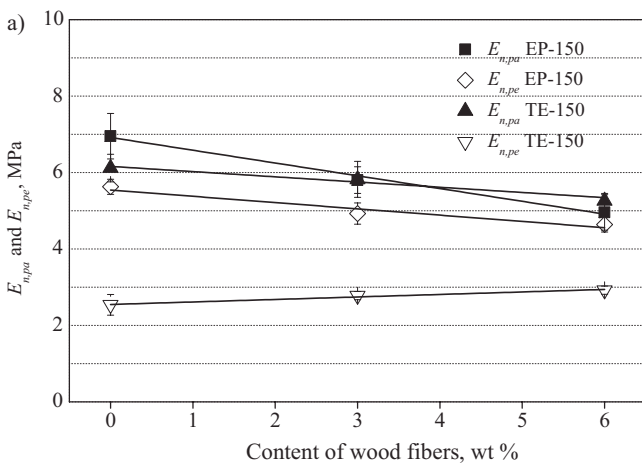
Fig. 9. Normalized Young's modulus in parallel direction ( E_{n,pa} ) and in perpendicular direction ( E_{n,pe} ) of rigid PUR-PIR foams modified with wood fibers; isocyanate index: a) 150, b) 250 (data, taking into account apparent density of foams, normalized according to [23])
