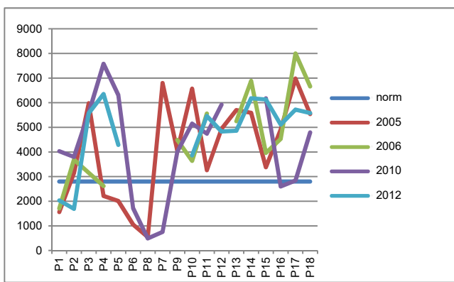
Fig. 5. Spatial and temporal variation of electrical conductivity (EC); P1–P18 = measurement points as in Fig. 3; source: own study
