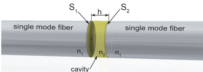
Fig. 1. Optical fiber Fabry–Pérot interferometer: h – length of the cavity, n_1 – refractive index of the fiber core, and n_2 – refractive index of the medium in the cavity.
