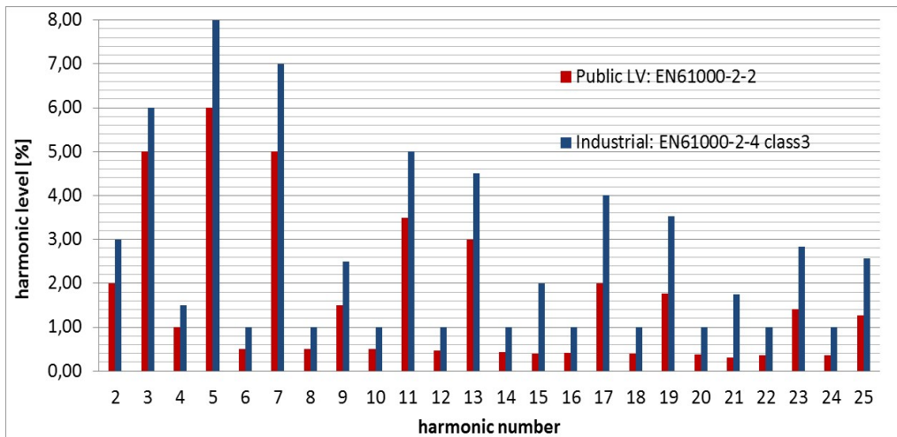
Fig. 2. Minimum requirements for harmonic immunity – compatibility levels
