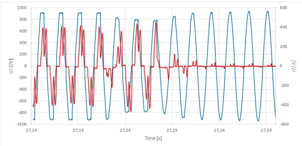
Fig. 4. Waveforms of the instantaneous value of current and voltage at the terminals of the converter point of common coupling during a dip
