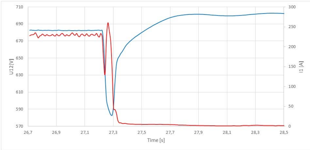
Fig. 3. Waveform of root-mean-square current and voltage at the terminals of the converter point of common coupling during a dip
