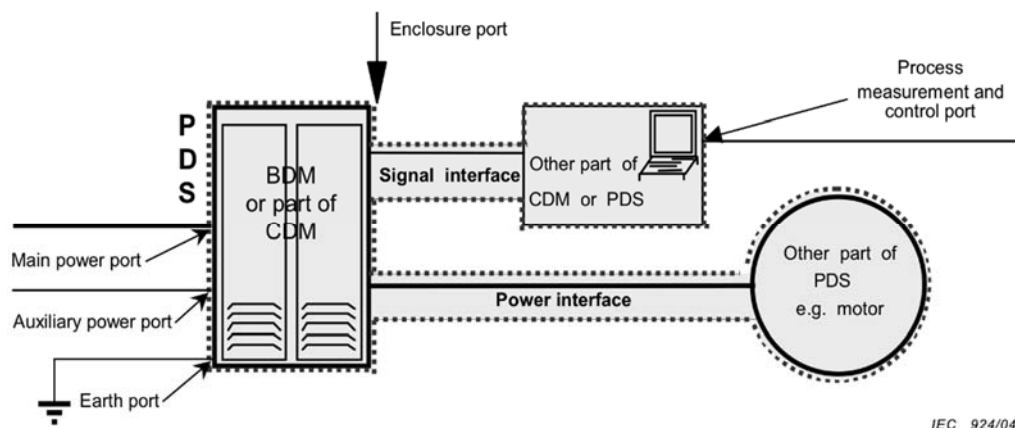
Fig. 1. Internal interfaces of the PDS and examples of ports according to standard [1]
