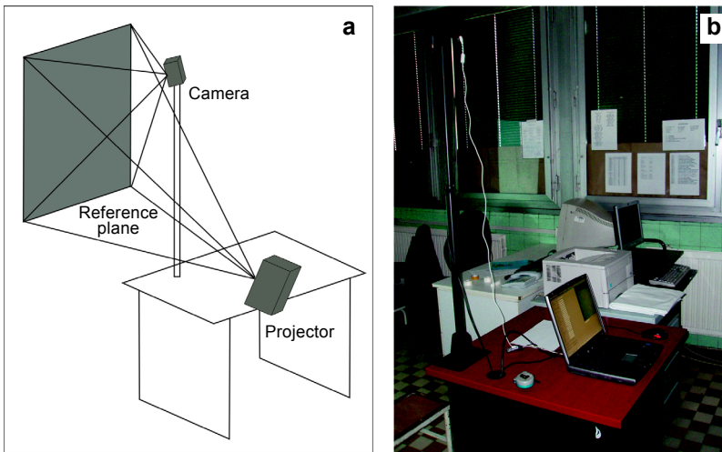
Fig. 2. Optical layout of the electronic moiré equipment (a). Operating equipment (b).
