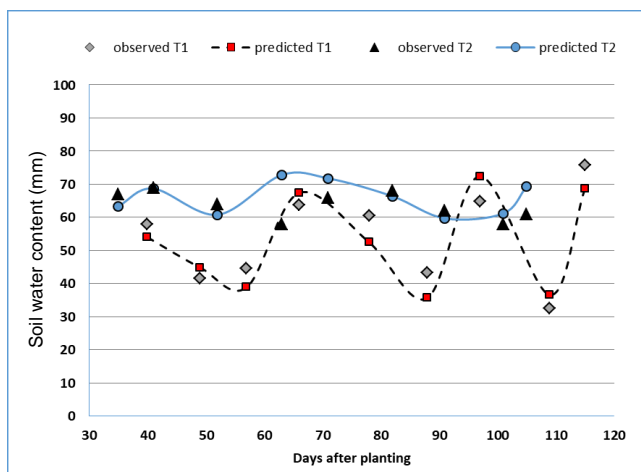
Fig. 7. Simulated and measured soil water content against days of potato transplanting for AquaCrop model validation (2017/2018); T1 and T2 as in Fig. 1; source: own study
