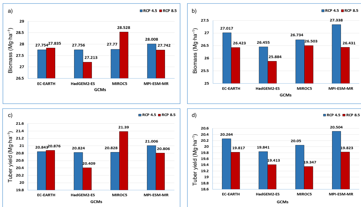
Fig. 9. Simulated parameters at harvest for a potato with global climate models under RCP 4.5 and 8.5: a) biomass 2030s, b) biomass 2050s, c) tuber yield 2030s, d) tuber yield 2050s; source: own study
