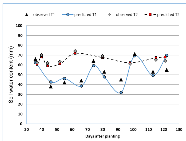
Fig. 4. Simulated and observed soil water content against days of potato transplanting for AquaCrop model calibration (2016/2017); T1 and T2 as in Fig. 1; source: own study
