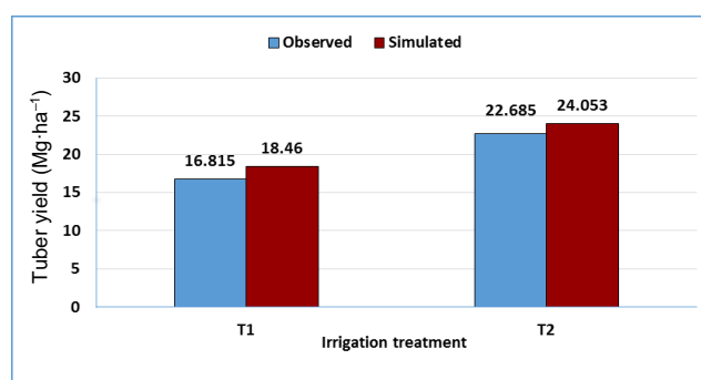
Fig. 3. Simulated and measured tuber yield of potato under both irrigation treatments for AquaCrop model calibration (2016/2017); T1 and T2 as in Fig. 1; source: own study
