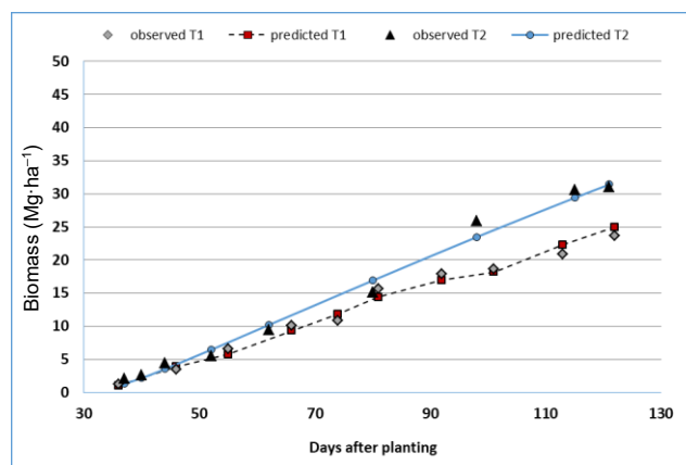
Fig. 2. Simulated and measured above ground biomass in potato against days after transplanting as a result of the AquaCrop model calibration (2016/2017); T1 and T2 as in Fig. 1; source: own study
