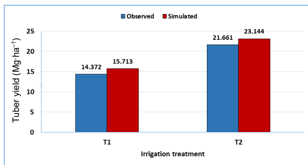
Fig. 8. Simulated and measured potato tuber yield for AquaCrop model validation (2017/2018); T1 and T2 as in Fig. 1; source: own study
