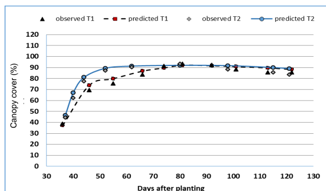
Fig. 1. Simulated and measured canopy cover against days of potato transplanting for AquaCrop model calibration (2016/2017); T1 = irrigation at 50% of field capacity, T2 = irrigation at 80% of field capacity; source: own study
