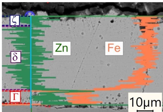
Fig. 4. The linear EDS analysis at the zinc coating cross section deposited on steel after the HT – 460°C
