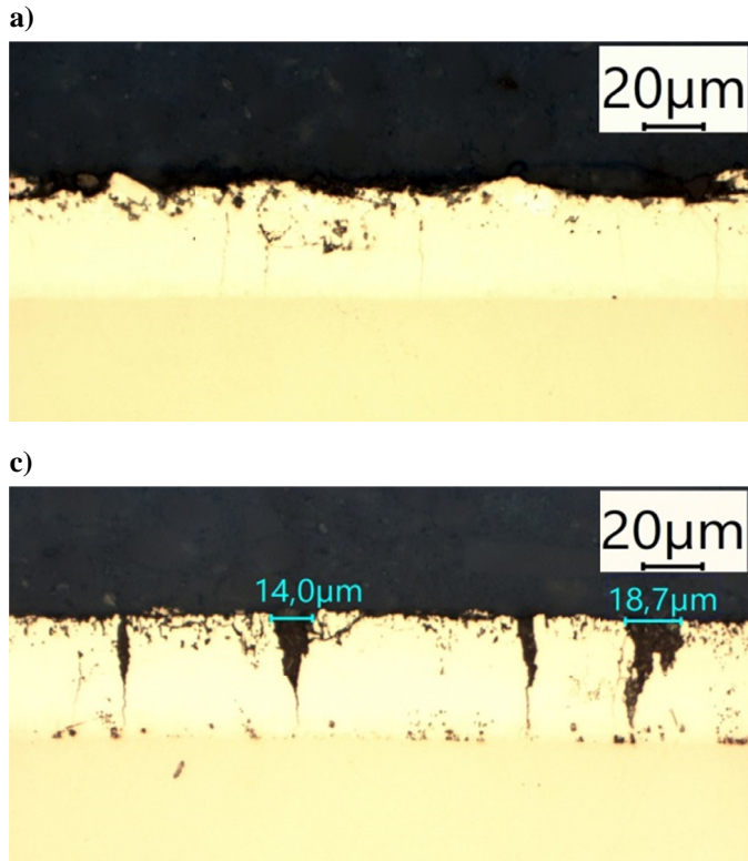
Fig. 3. The microstructure observed at the cross section of zinc coating deposited on steel after the HT – a (430°C), b (460°C), c (530°C) and cast iron – d (530°C)
