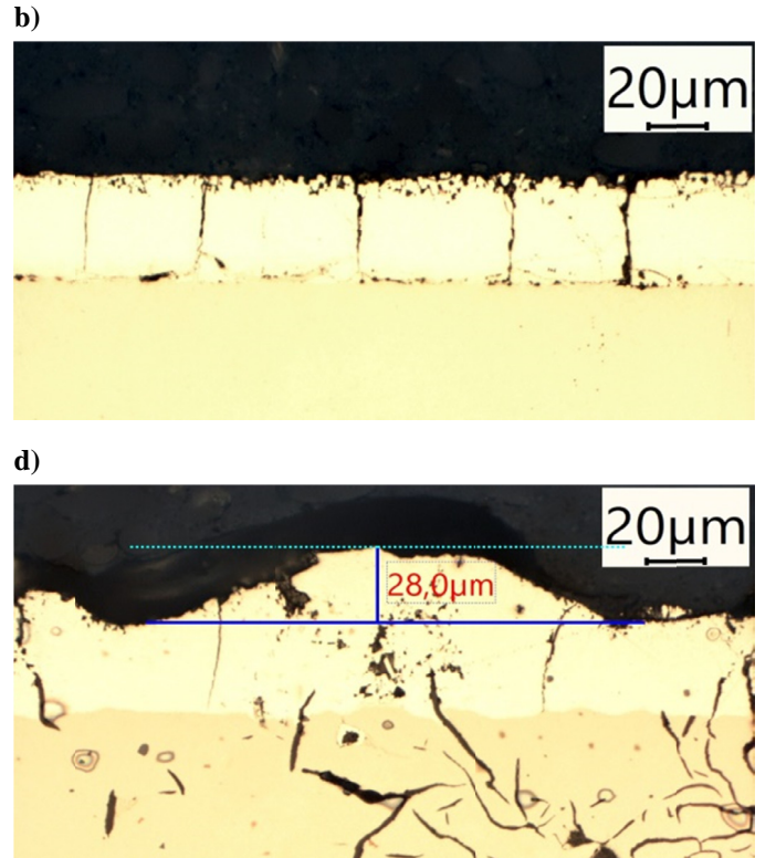
Fig. 3. The microstructure observed at the cross section of zinc coating deposited on steel after the HT – a (430°C), b (460°C), c (530°C) and cast iron – d (530°C)
