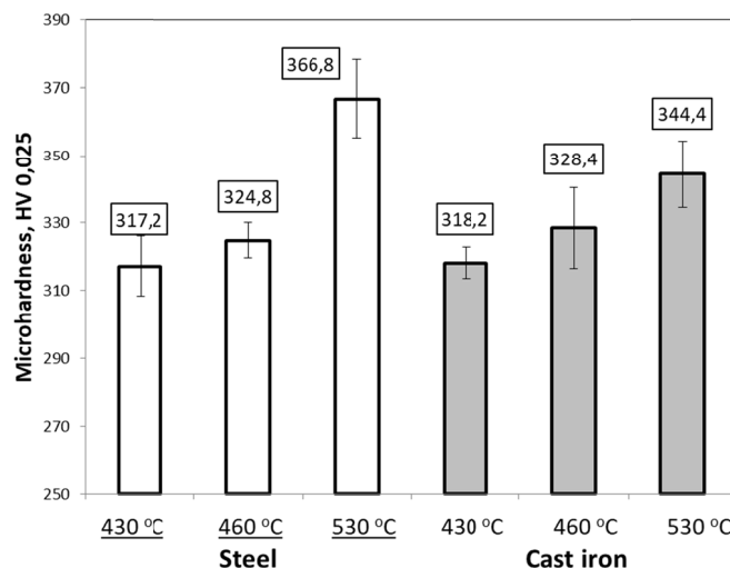
Fig. 5. The microhardness measured on the outer zinc coating surface after HT deposited on steel and cast iron
