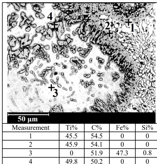
Fig. 6. Point EDS analysis (%wt.) - casting with an empty insert connector and dimensions 70x100x120 mm
