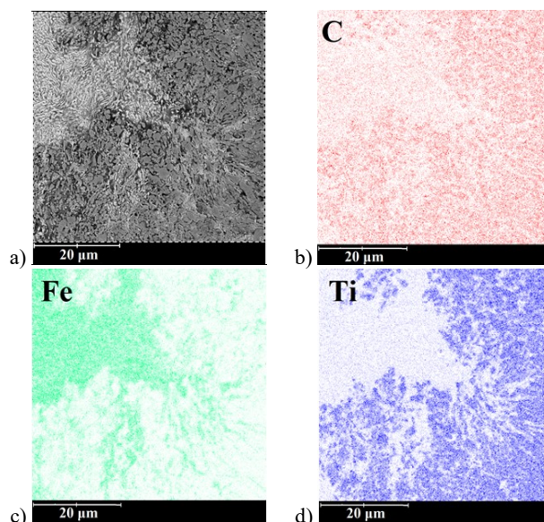
Fig. 7. Surface EDS analysis of the titanium layer - insert with a full connector, casting dimensions: 70x100x160 mm; a) microstructure of the surface, b) carbon content, c) iron content, d) titanium content
