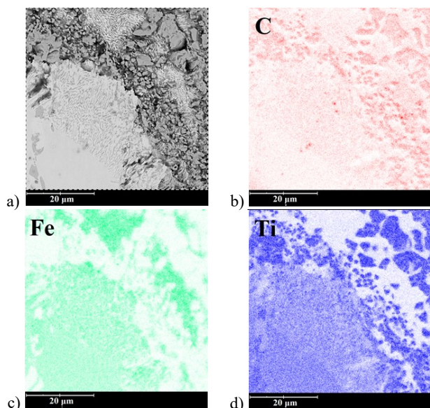
Fig. 8. Surface EDS analysis of the titanium layer - insert with an empty connector, casting dimensions: 70x100x160 mm; a) microstructure of the surface, b) carbon content, c) iron content, d) titanium content
