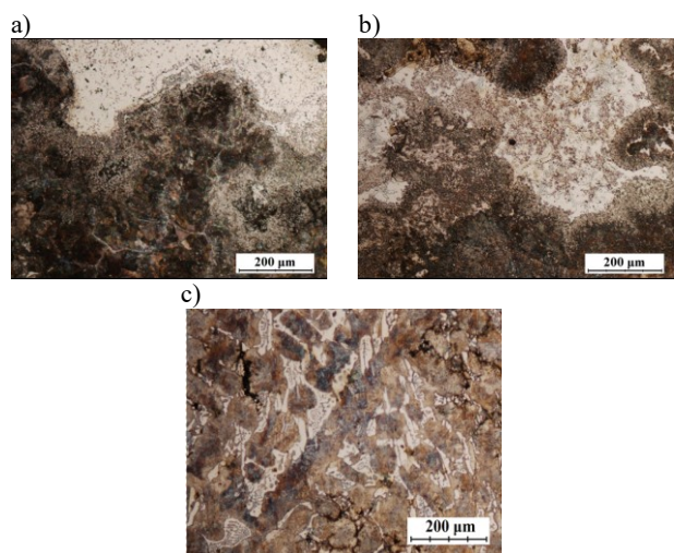
Fig. 4. The area of carbides precipitation in casting with empty connector; magnification 100x; casting thickness: a) 160 mm; b) 120 mm; c) 80 mm
