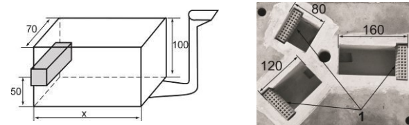
Fig. 2. Shape of the casting with dimensions; 1- titanium insert
