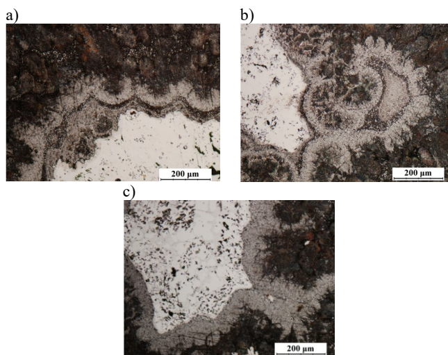
Fig. 3. The area of carbides precipitation in casting with full connector; magnification 100x; casting thickness: a) 160 mm; b) 120 mm; c) 80 mm
