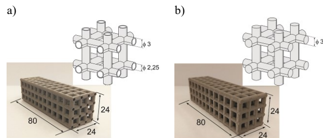
Fig. 1. 3D printed insert; a) with an empty connector; b) with a full connector
