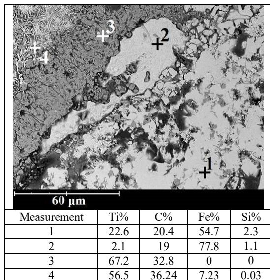
Fig. 5. Point EDS analysis (%wt.) - casting with an empty insert connector and dimensions 70x100x160 mm
