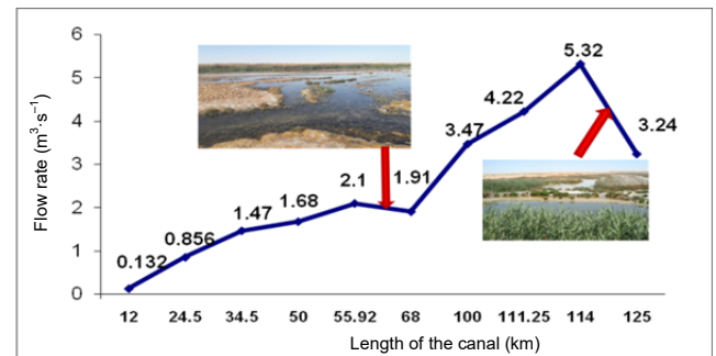
Fig. 3. Variation of the flow according to the length of the channel; source: own elaboration
