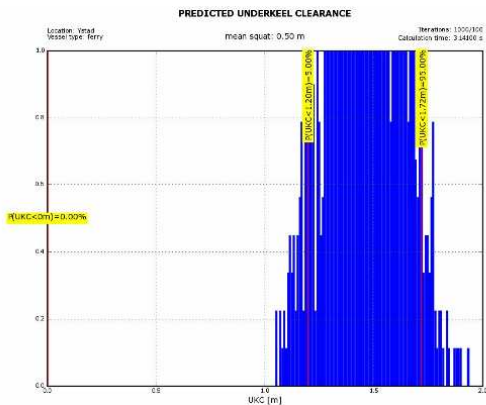
Figure 5.a. Histogram UKC and squat value 130m before heads /sea wave =0,4 m/
