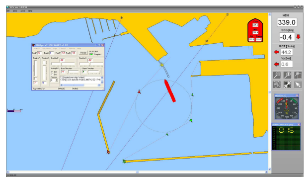
Figure 3. Interface of simulation model ferry entering to Ystad
