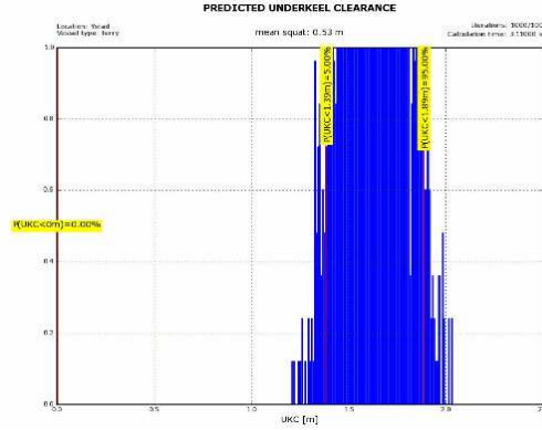
Figure 5.b. Heads: Histogram UKC and squat value /sea wave =0,2 m/
