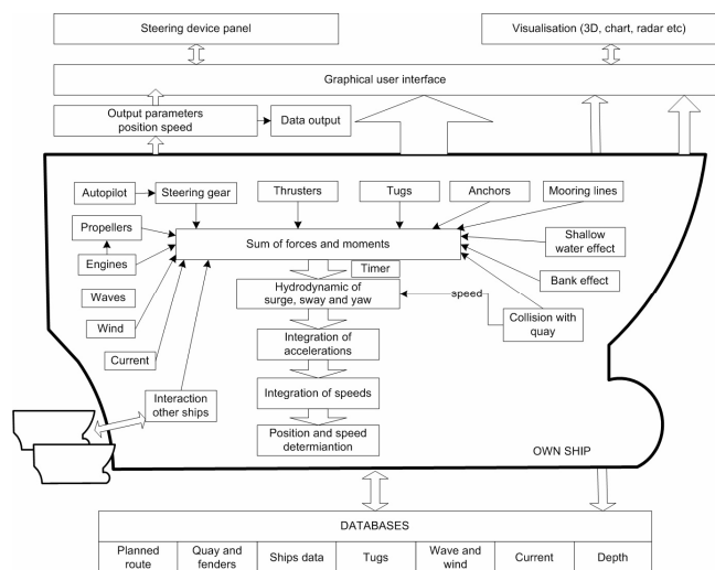
Figure 1. The main diagram of simulation model
