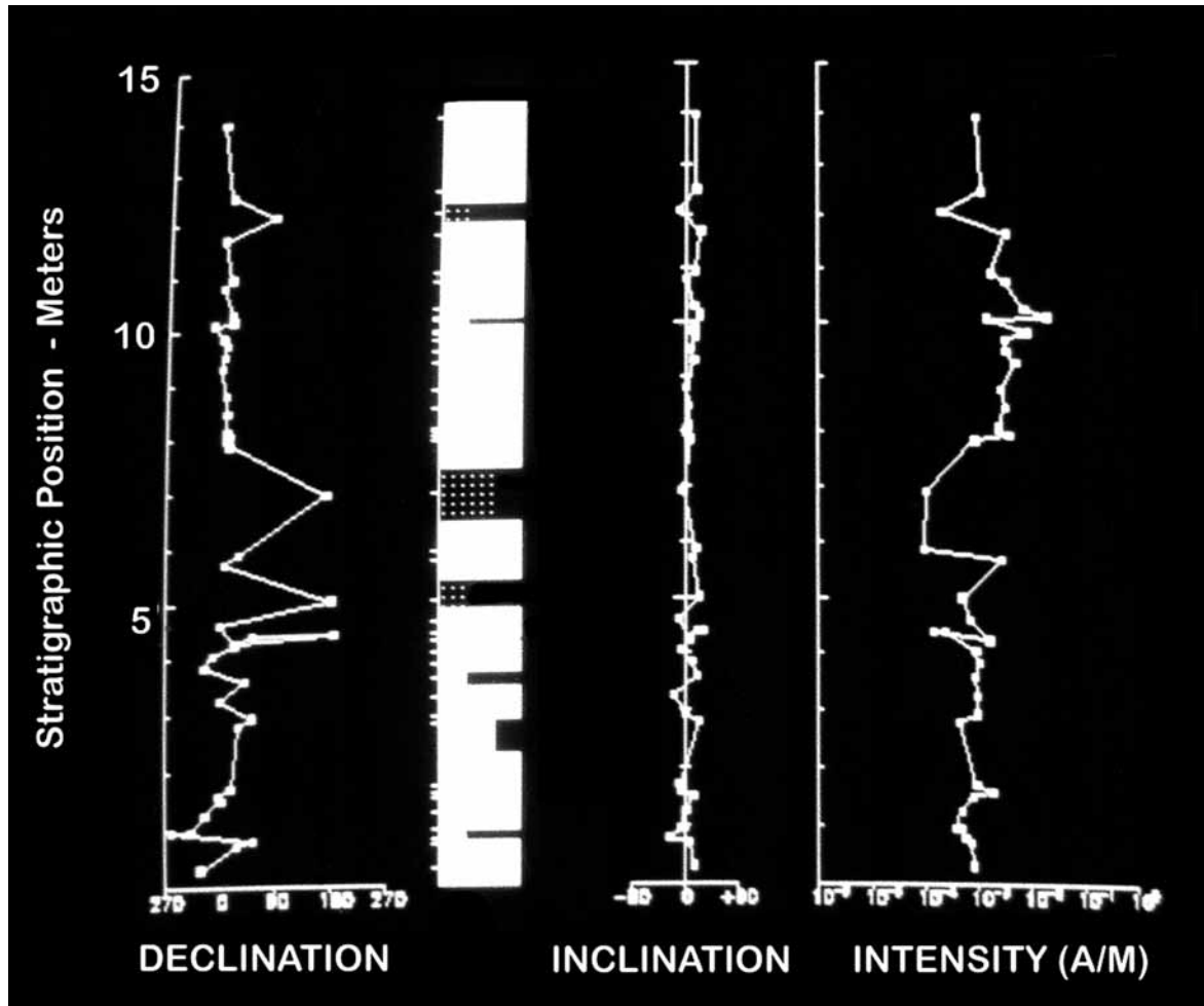
Fig. 6. Magnetostratigraphic plot of the Tenney Canyon Tongue
