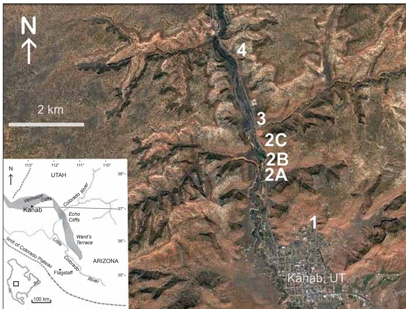
Fig. 1. Location map, showing the Kayenta sampling sites of this study
