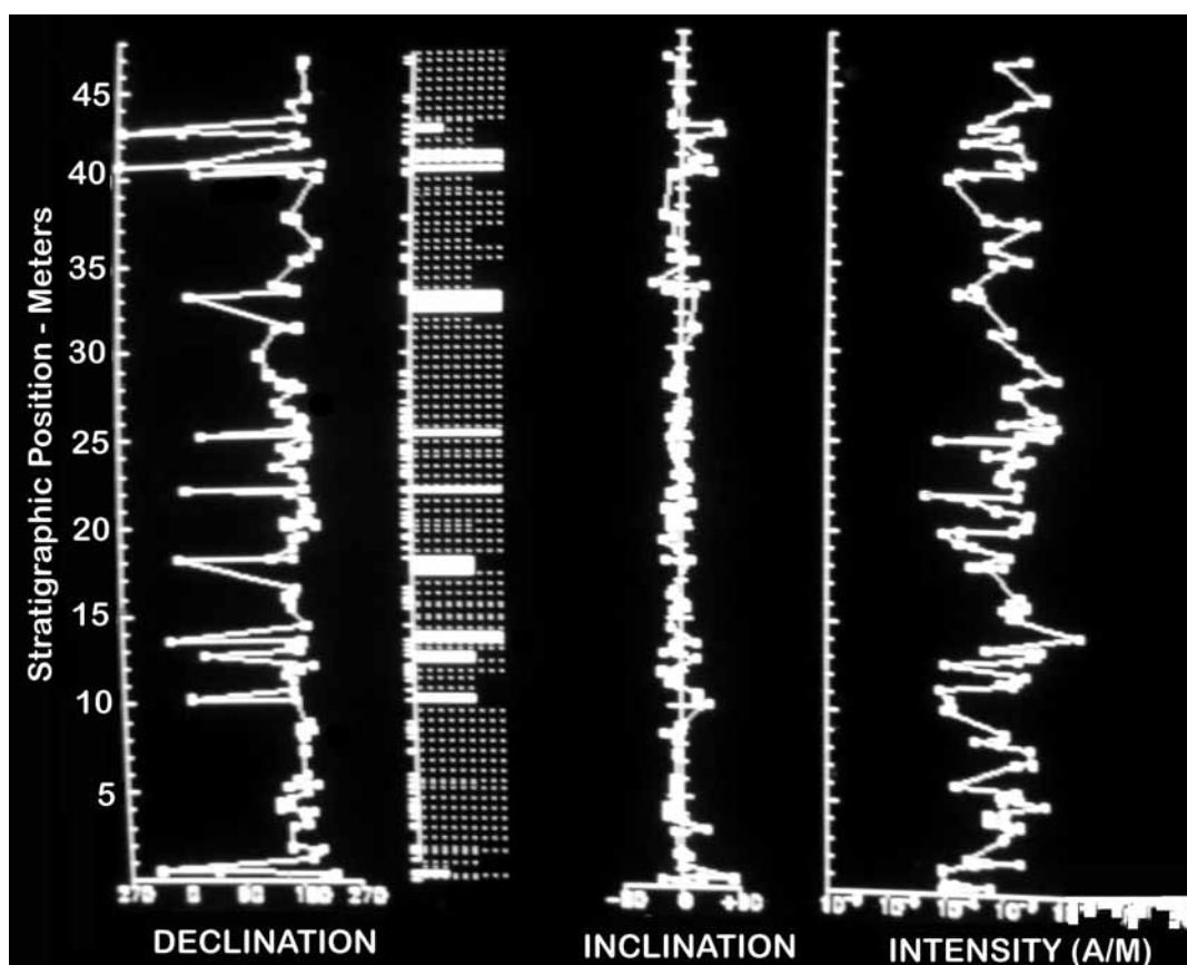
Fig. 4. Magnetostratigraphic plot of the Kayenta Formation.
