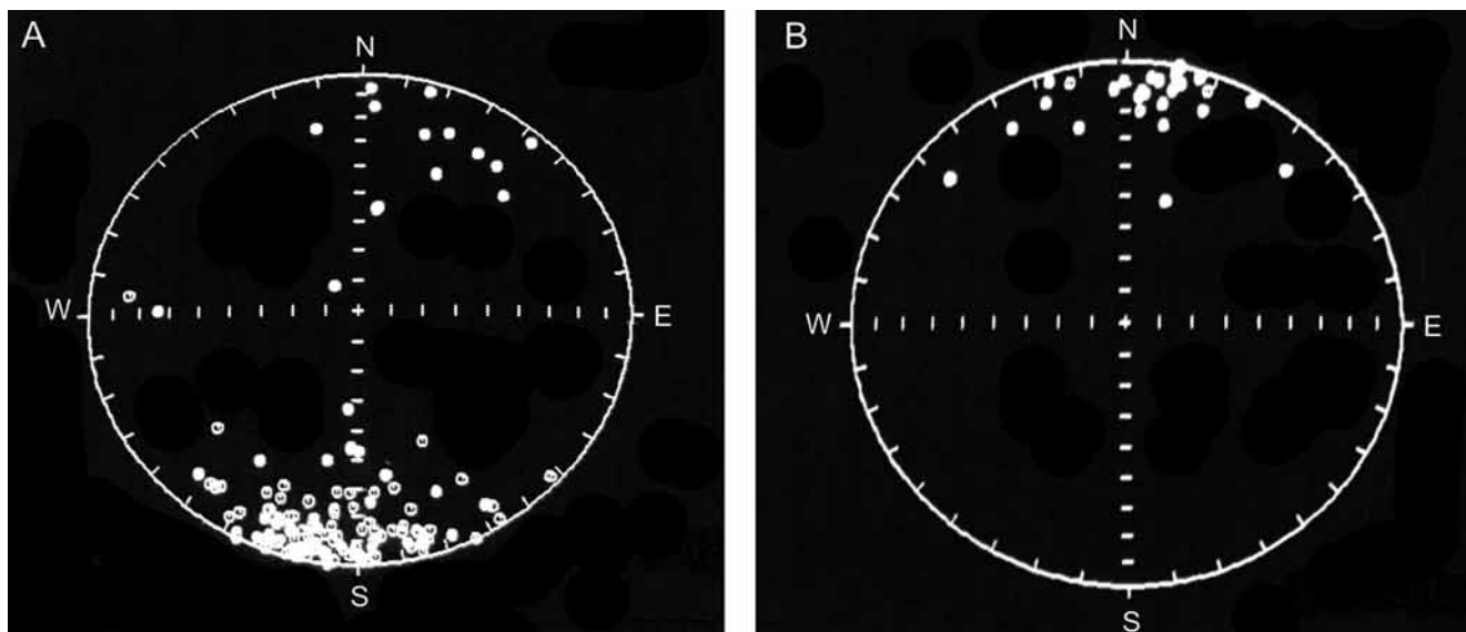
Fig. 3. Equal area stereographic plots of the demagnetized directions of the Kayenta Formation (A) and the Tenney Canyon Tongue (B). Open circles are upper hemisphere directions; solid circles are lower hemisphere directions.
