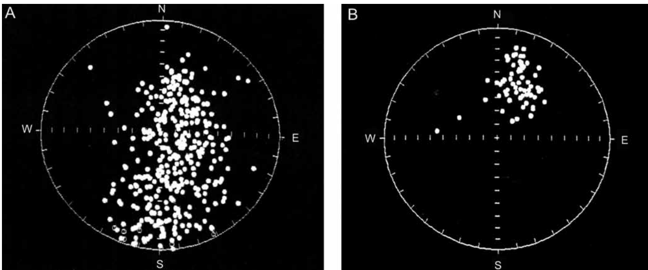
Fig. 2. Equal area stereographic plots of the natural remanent magnetization directions of the Kayenta Formation (A) and of the Tenney Canyon Tongue (B)
