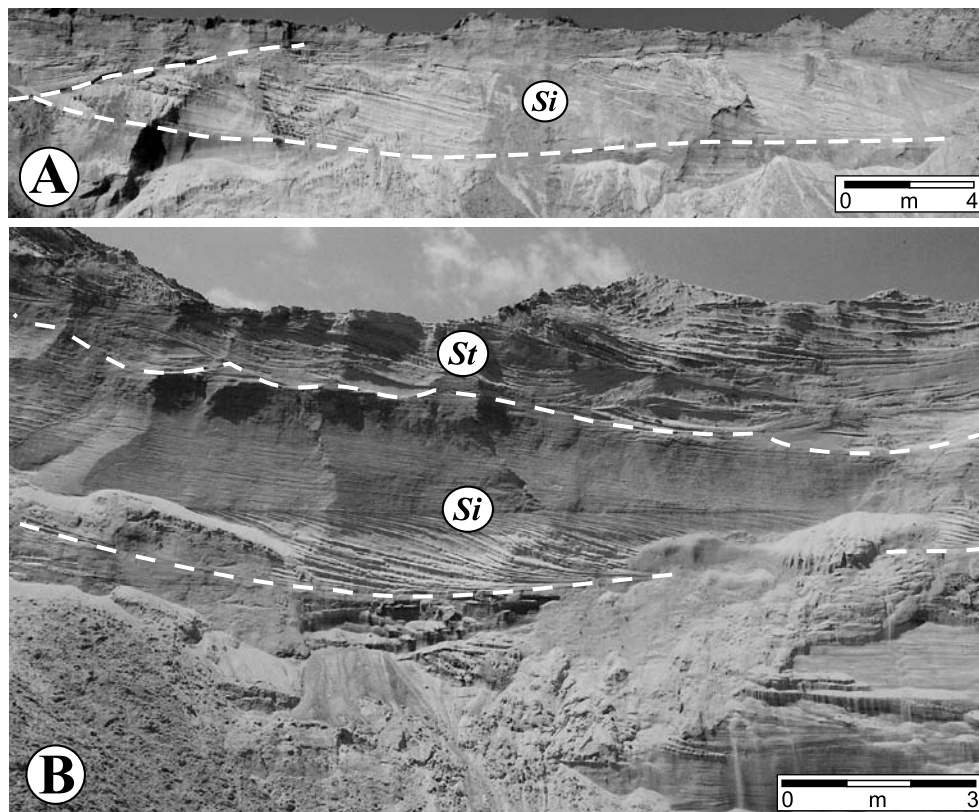
Fig. 5. Two examples of palaeochannels from unit 1. A - Palaeochannel filled with a thick sandy package derived from a side bar; B - Two stacked palaeochannel infills. The lower infill was deposited by laterally accreted side bars ( Si ) and the upper one by 3-D dunes ( St ).
