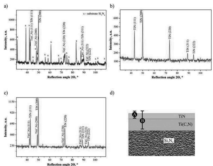
Fig. 1. X-ray diffraction pattern of Ti(C,N)+TiN coating deposited on the sialon ceramics obtained by a) Bragg-Brentano method, b, c) GIXRD method ( \alpha = 0.5 and 3^\circ ), d) Scheme of packing layers into Ti(C,N)+TiN coating, which was deposited on sialon tool ceramic with marking depths of GIXRD phase analysis: A for \alpha = 0.5^\circ , B for \alpha = 3^\circ
