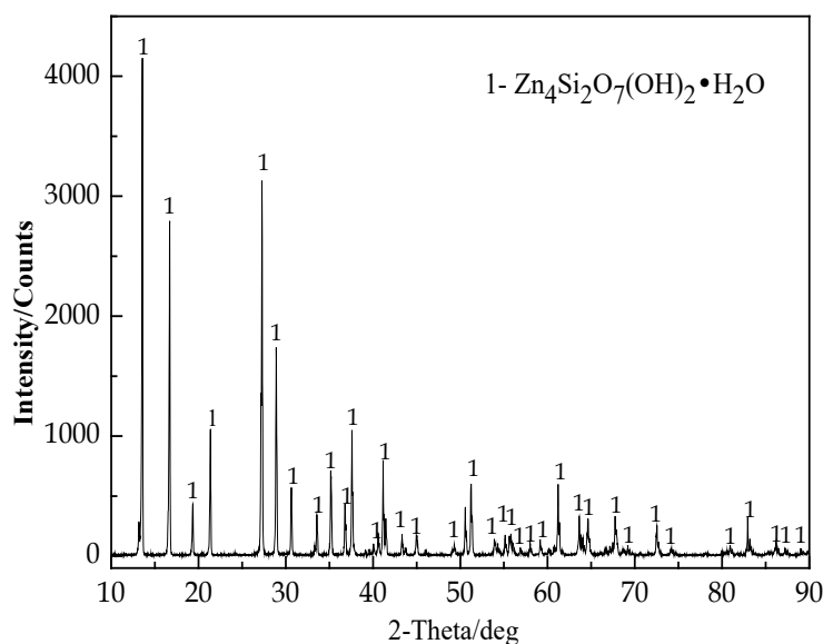
Fig. 1. XRD pattern of pure hemimorphite samples
