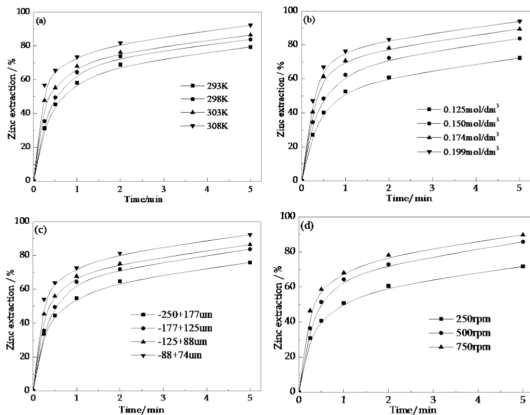
Fig. 2. Effect of operation parameters on the leaching efficiency of Zinc: (a) temperature, (b) MSA concentration, (c) particle size, (d) stirring speed
