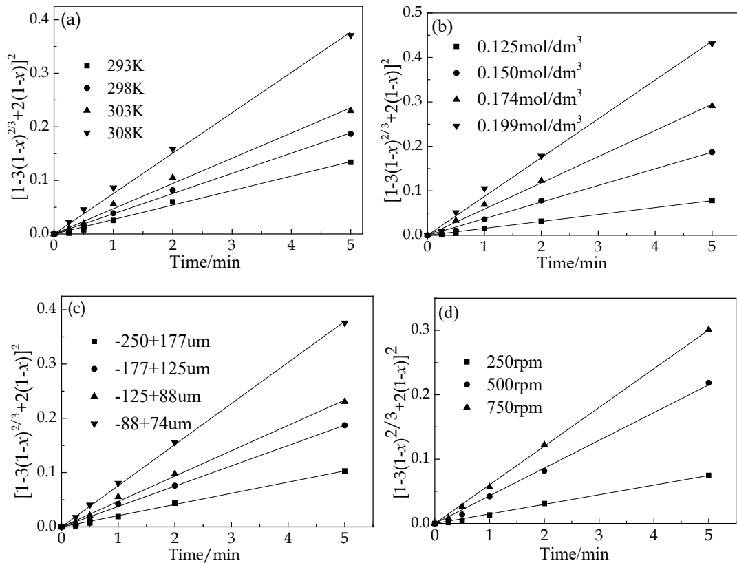
Fig. 3. Plot of [1-3(1-x)^{2/3}+2(1-x)]^2 vs. time for different operation parameters: (a) temperature, (b) MSA concentration, (c) particle size, and (d) stirring speed
