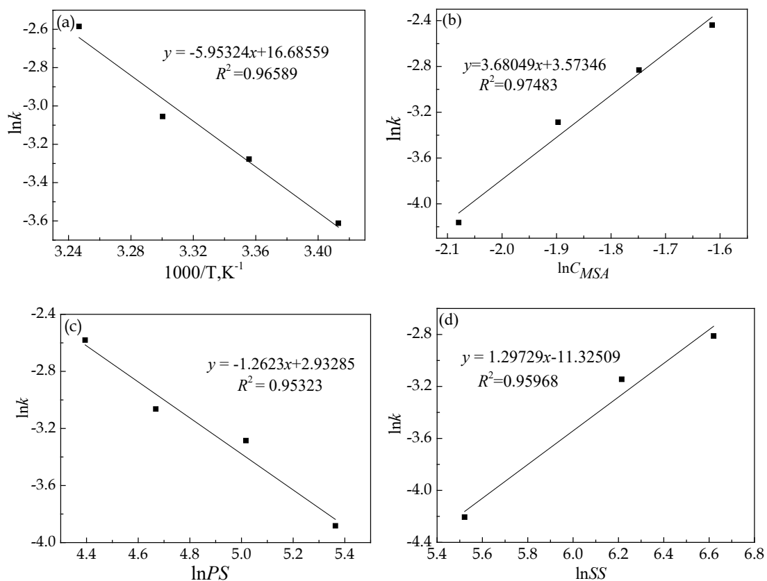
Fig. 4. Plot of \ln k versus operation parameters: (a) temperature, (b) MSA concentration, (c) particle size, and (d) stirring speed
