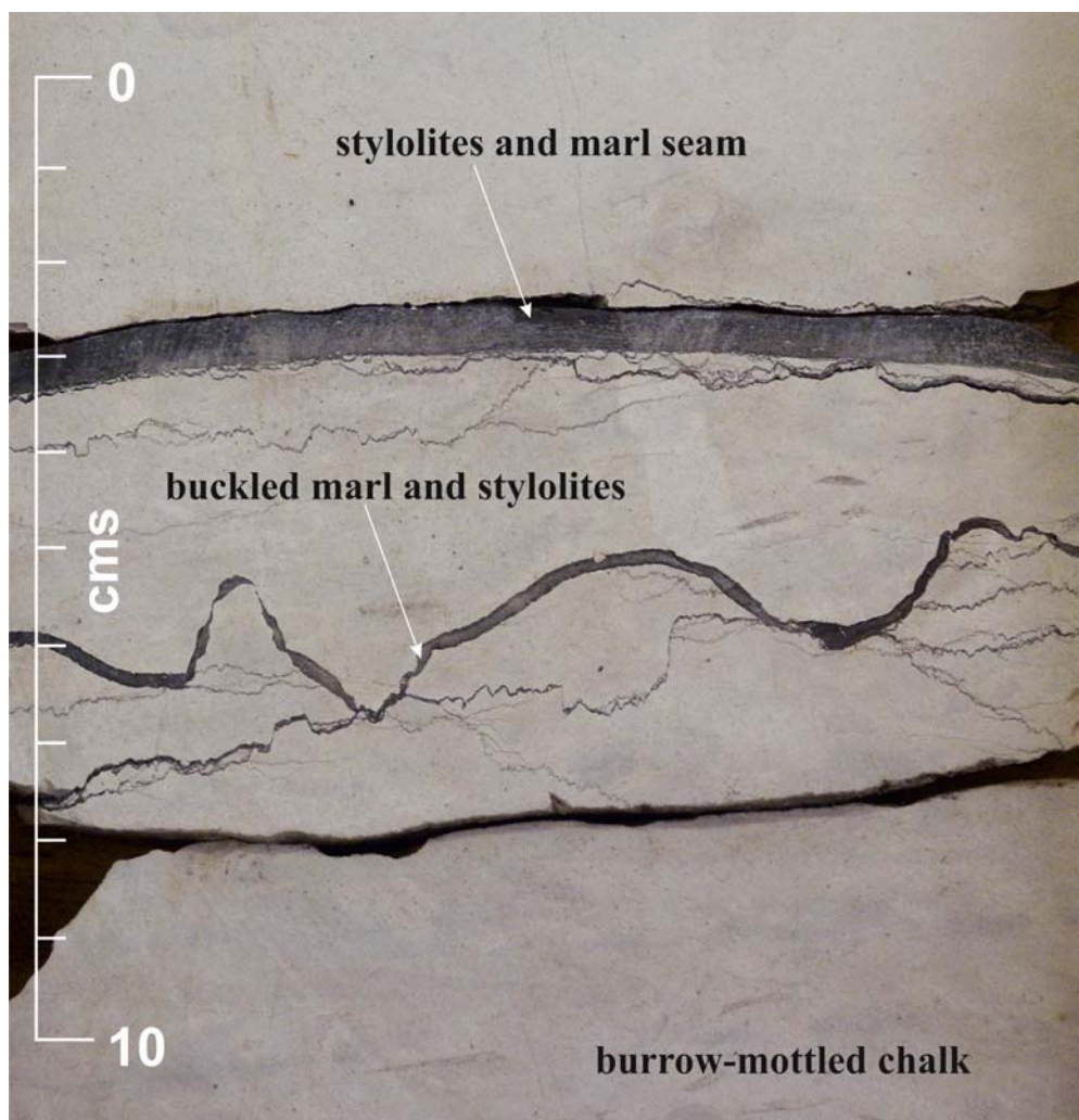
Text-fig. 25. High density white chalk ( SG > 1.95 ) from the North Sea showing primary marl seams that have been secondarily compressed and buckled in association with the development of syn-deformational stylolites and secondary marl seams. (from Mortimore, 2014, figure 5.37)
