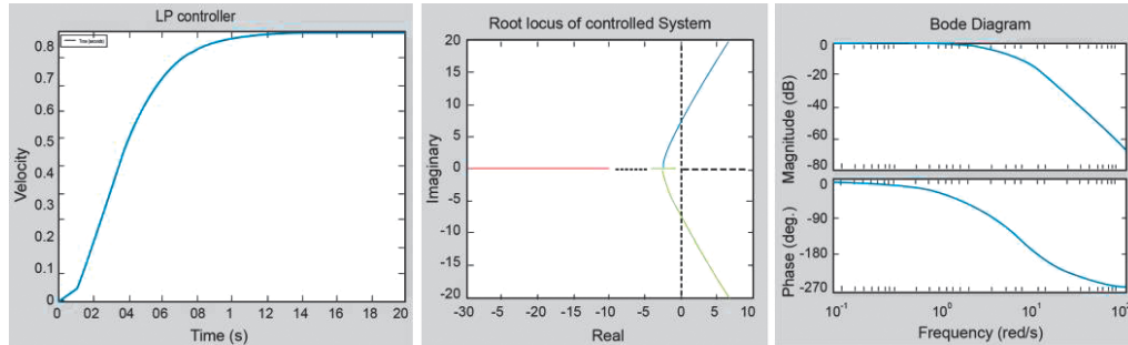
Fig. 10. Step response, root locus, and Bode plot of DC motor system angular velocity using an LQR controller
