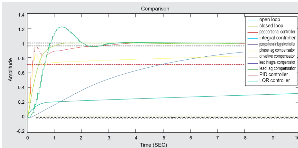
Fig. 11. Comparison among all strategies used to control step response of DC motor system angular velocity
