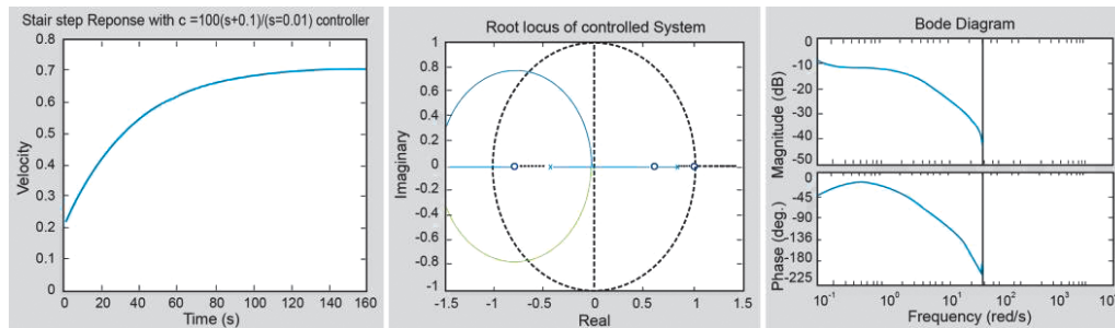
Fig. 9. Step response, root locus, and Bode plot of DC motor system angular velocity using a lead lag compensator
