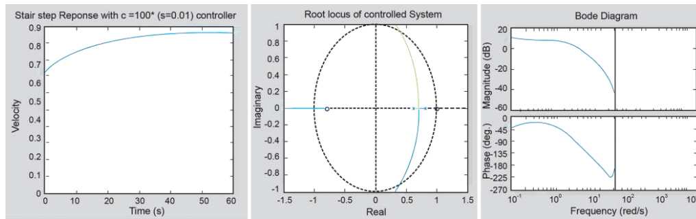
Fig. 7. Step response, root locus, and Bode plot of DC motor system angular velocity using a phase lag compensator
