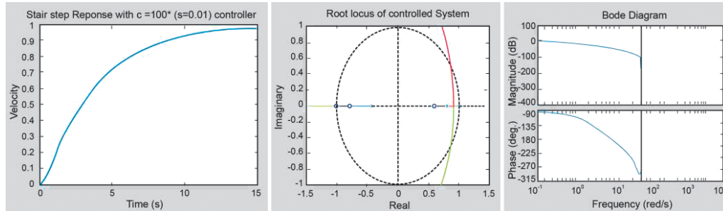
Fig. 8. Step response, root locus, and Bode plot of DC motor system angular velocity using a lead integral compensator
