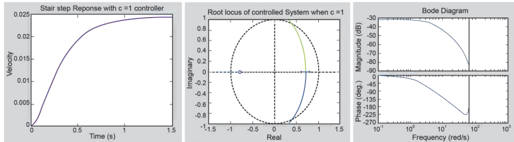
Fig. 1. Step response, root locus, and Bode plot of closed loop DC motor system angular velocity
