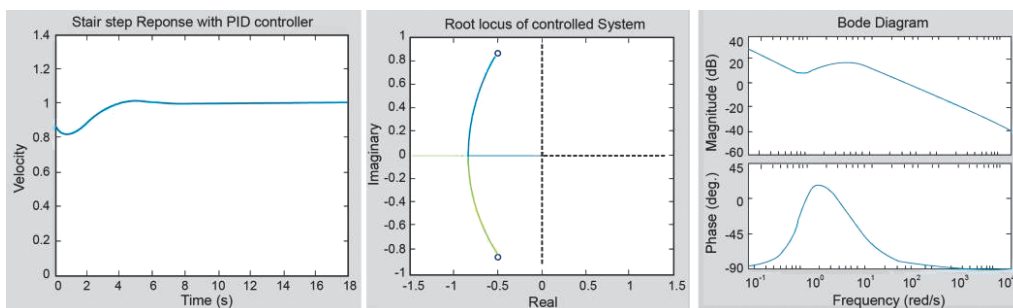
Fig. 6. Step response, root locus, and Bode plot of DC motor system angular velocity using a PID controller
