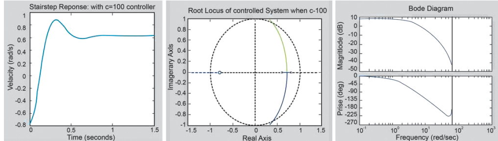
Fig. 2. Step response, root locus, and Bode plot of DC motor system angular velocity when c = 100
