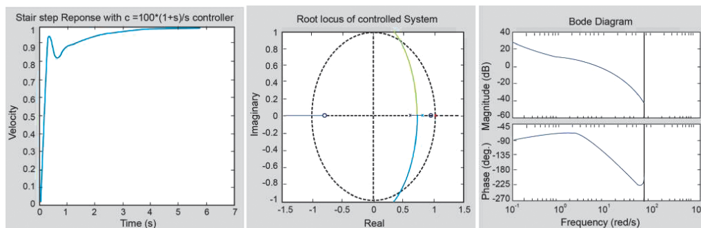
Fig. 4. Step response, root locus, and Bode plot of DC motor system angular velocity using a PI controller
