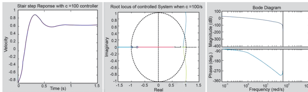
Fig. 3. Step response, root locus, and Bode plot of DC motor system angular velocity using an integral controller
