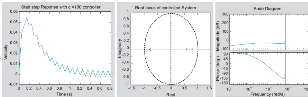
Fig. 5. Step response, root locus, and Bode plot of DC motor system angular velocity using a derivative controller
