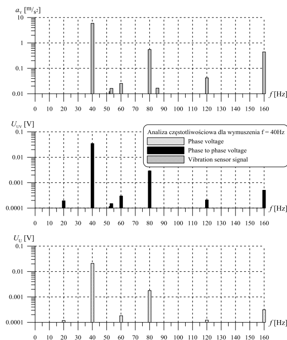
Fig. 7. The frequency analysis of signals: own and vibration sensor
