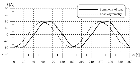
Fig. 10. Current with symmetry and asymmetry point operation – the result of laboratory tests
