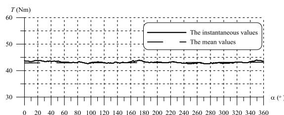
Fig. 1. Electromagnetic torque for generator loaded symmetrically
