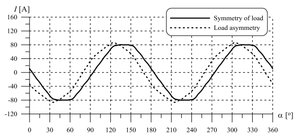
Fig. 8. Current with symmetry and asymmetry point operation – the result of simulation
