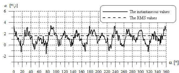
Fig. 5. Vibration acceleration for generator loaded asymmetrically (the current in one phase I = 0,75 I_n )
