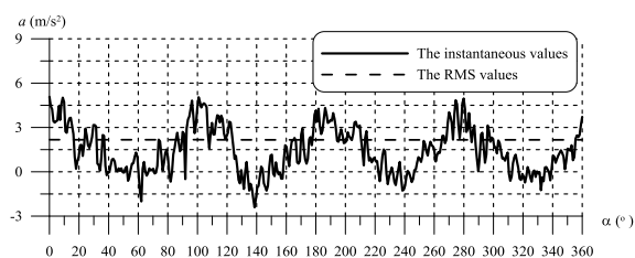
Fig. 6. Vibration acceleration for generator loaded asymmetrically (the break in one phase)
