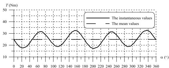
Fig. 3. Electromagnetic torque for generator loaded asymmetrically (the break in one phase)
