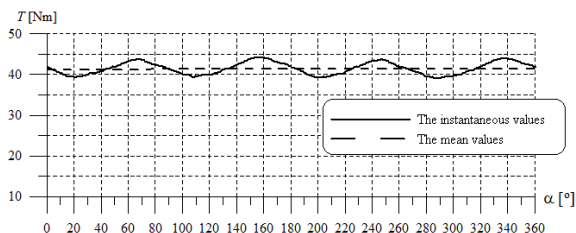
Fig. 2. Electromagnetic torque for generator loaded asymmetrically (the current in one phase I = 0,75 I_n )
