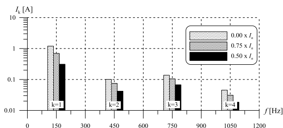
Fig. 12. Current for several asymmetries of point operation
