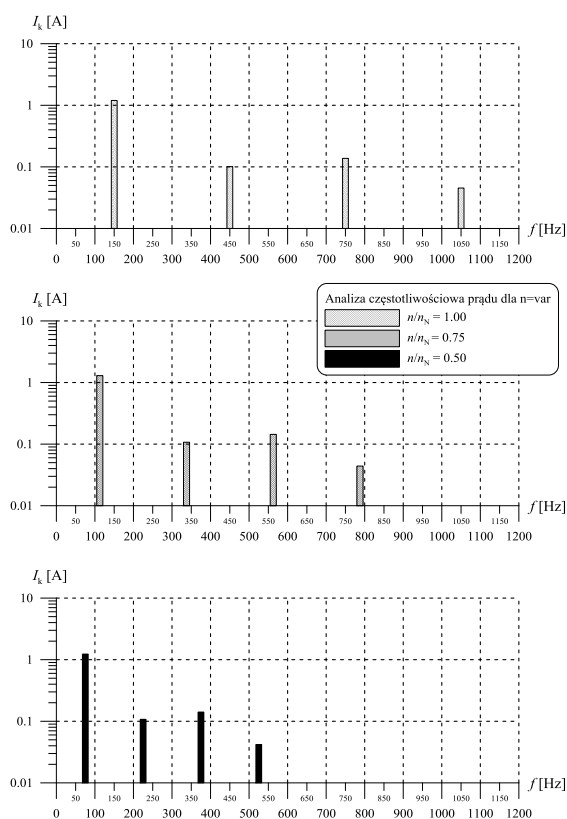
Fig. 13. The frequency analysis of generator current for several rotational speeds
