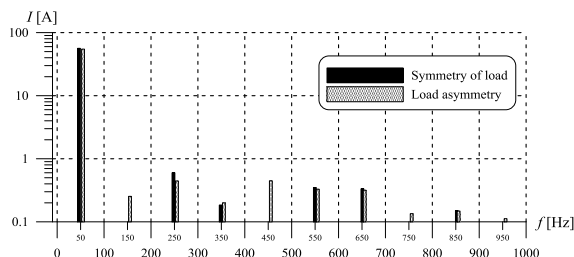
Fig. 11. Current with symmetry and asymmetry point operation – the result of laboratory tests
