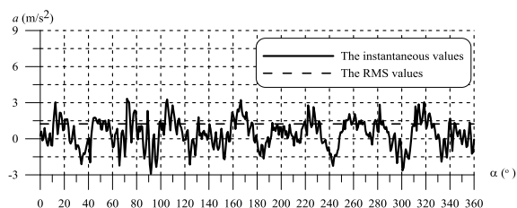
Fig. 4. Vibration acceleration for generator loaded symmetrically
