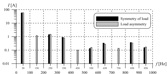
Fig. 9. Current with symmetry and asymmetry point operation – the result of simulation
