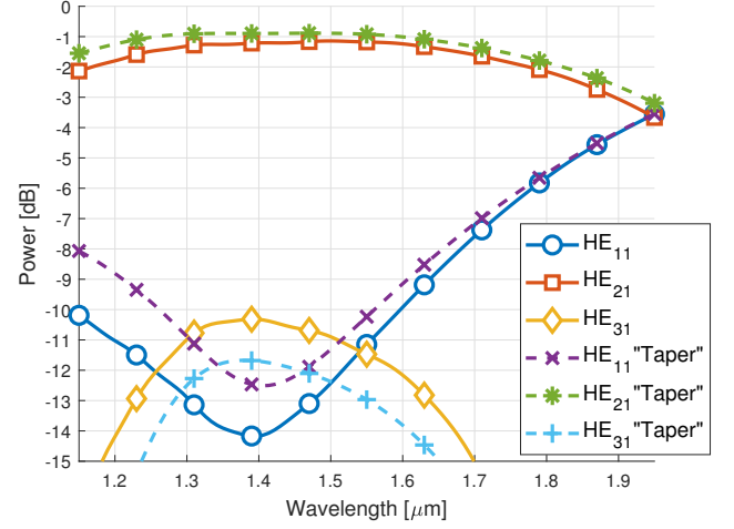
Fig. 4. Output power in \text{HE}_{11} , \text{HE}_{21} and \text{HE}_{31} modes vs. Wavelength
