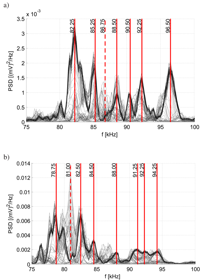
Fig. 11. Power spectral densities of ultrasonic signals registered at point B in the frequency range from 75 kHz to 100 kHz: a) specimen #1; b) specimen #2. Power spectral densities for the first ten signals ( n = 1-10 ) are marked with black lines
