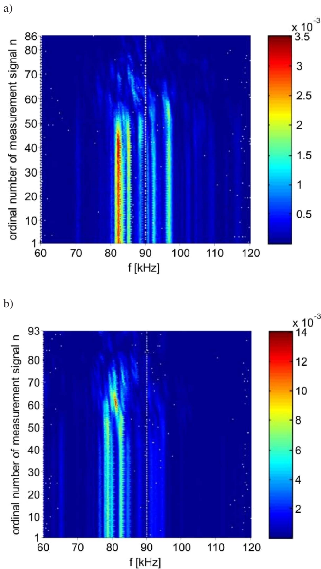
Fig. 10. Power spectral density maps of signals registered at point B: a) specimen #1; b) specimen #2 (power spectral densities are in units of (mV)^2/Hz )
