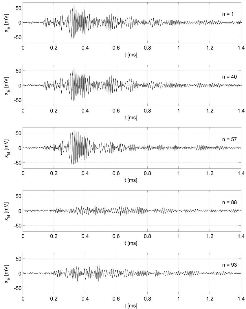
Fig. 7. Time signals registered at point B for different load levels for specimen #2
