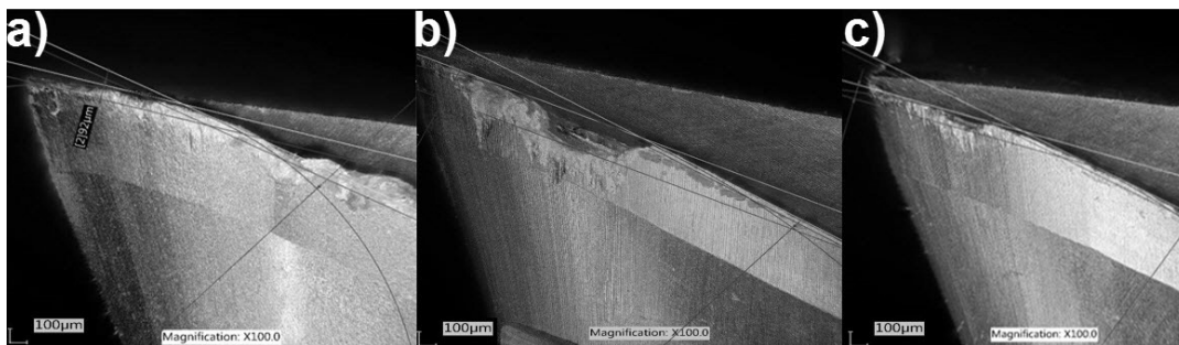
Fig. 2. Cutters blades after finishing the tests : a) milling cutter 1 - 5275.501nn, b) milling cutter 2 – C5275, c) milling cutter 3 – U5275
