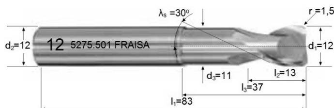
Fig. 1. View and dimensions of tools used during the tests
