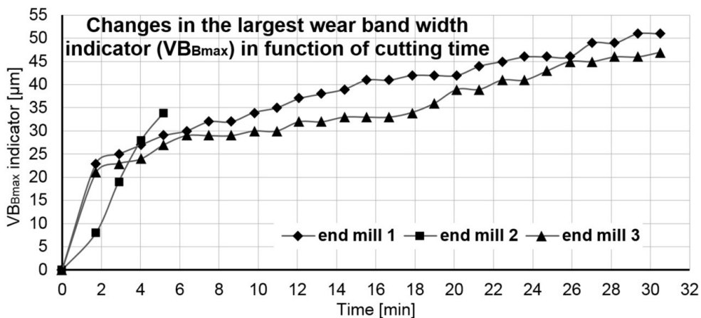
Fig. 4. Changes in the largest wear band width indicator ( VB_{Bmax} ) in function of cutting time
