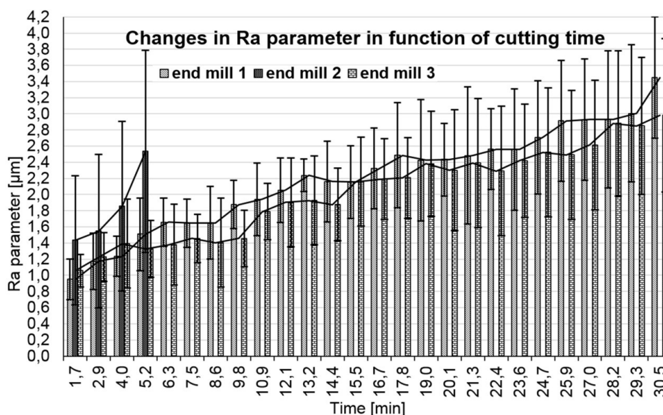
Fig. 5. Changes in Ra parameter in function of cutting time
