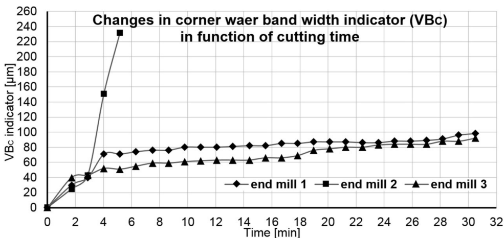
Fig. 3. Changes in corner wear band width indicator ( VB_C ) in function of cutting time
