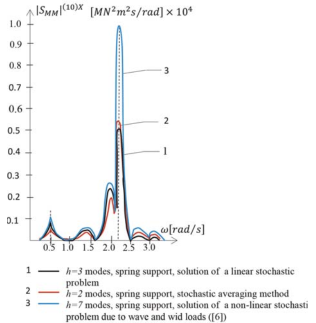
Fig. 5. Spectrum moduli of the response moment at the bottom at node 10 due to wave and wind loads
