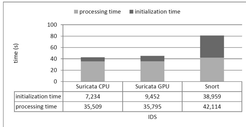
Fig. 3. Comparison of processing times of each IDS
