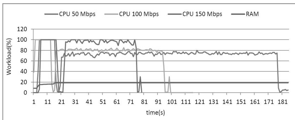
Fig. 5. Workload of system resources for IDS Suricata
